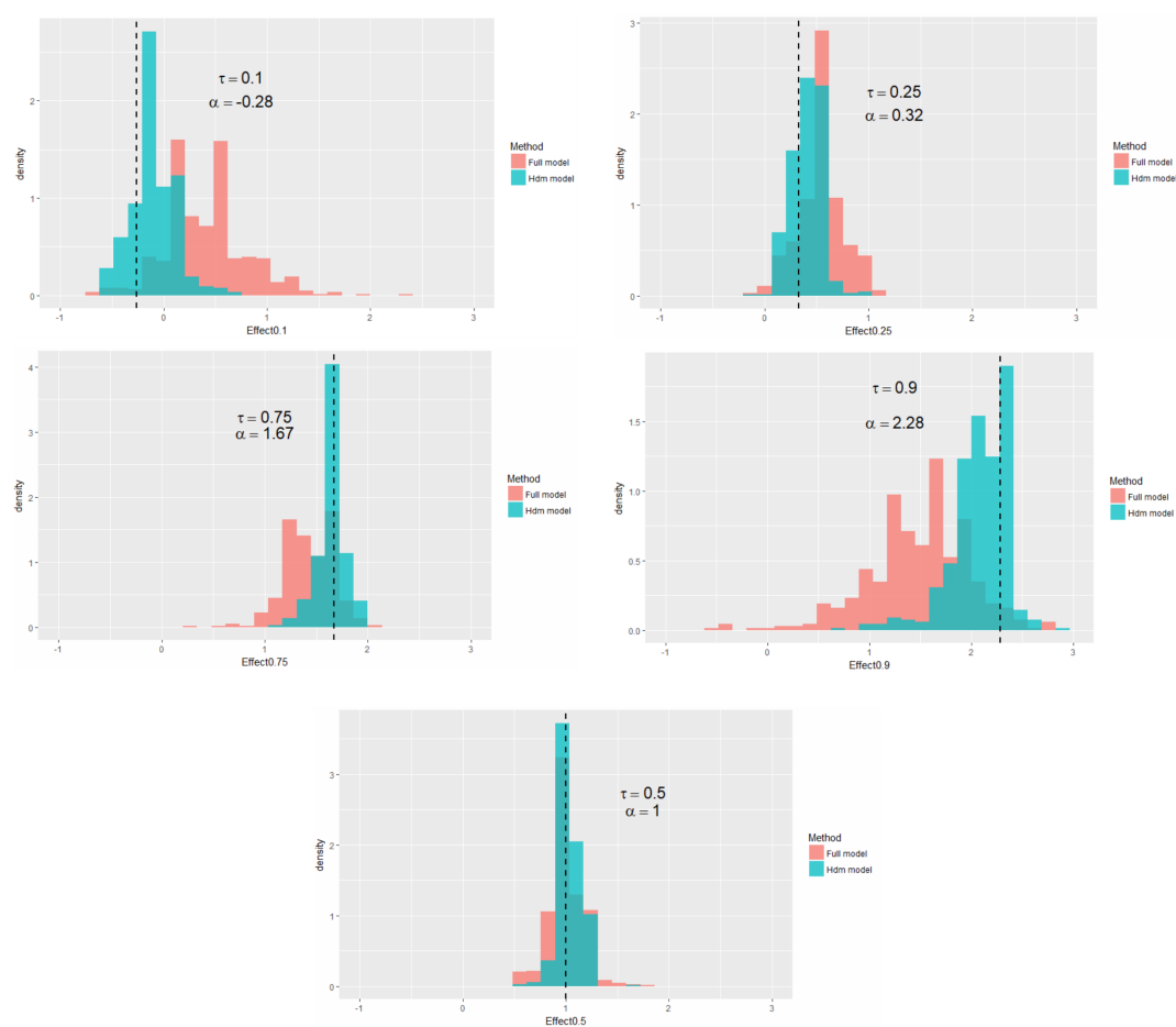
Figure 1. Histograms of the DML-IVQR Estimates (in green).
