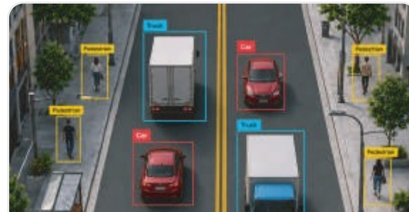
Object Classification
