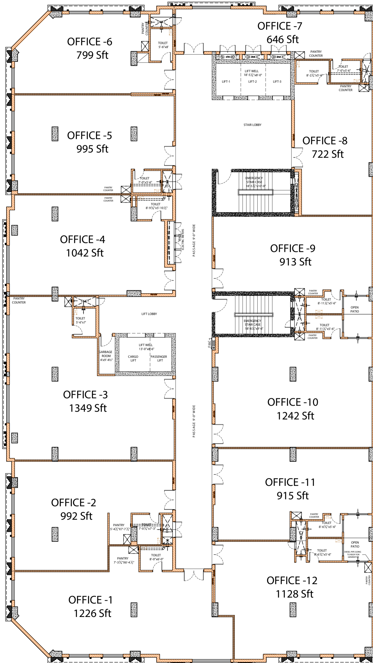
TYPICAL PLAN OF FLOOR 5,7, AND 9
