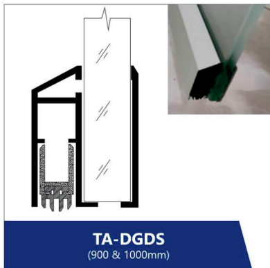
TA-DGDS (900 & 1000mm) Drop Down Seal for Frameless Glass Doors
