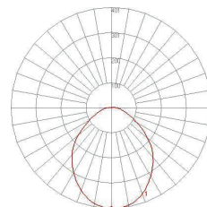
HDV 12W 4000K (963lm (Lamp), 400.8cd (Max intensity), 11W (Power))
