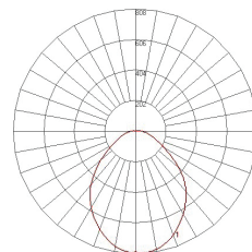
HDV 24W 4000K (1,891.3lm (Lamp), 807.5cd (Max intensity), 23W (Power))
