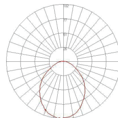
HDV 3W 4000K (241.5lm (Lamp), 102.2cd (Max intensity), 3W (Power))
