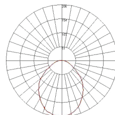
HDV 6W 4000K (490.3lm (Lamp), 204.7cd (Max intensity), 6W (Power))
