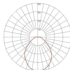
HDV 18W 4000K (1,327.8lm (Lamp), 566.3cd (Max intensity), 17W (Power))
