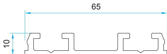
Code: P-1602 0,640 kg/m
