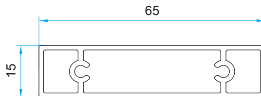
Code: P-1603 0,698 kg/m
