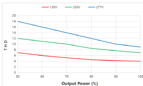
THD-Output Power Curve
