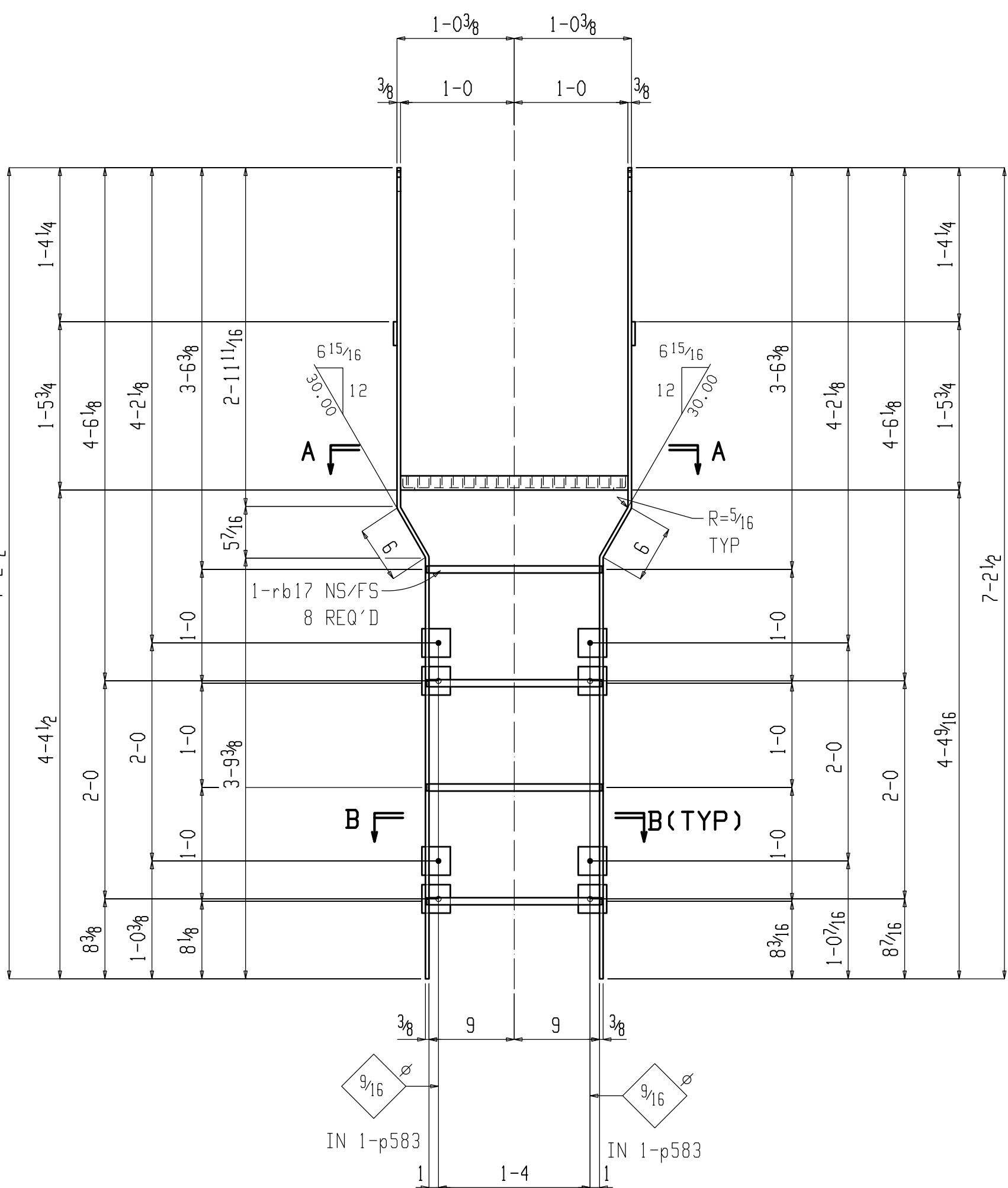
ONE LADDER 35LD1
