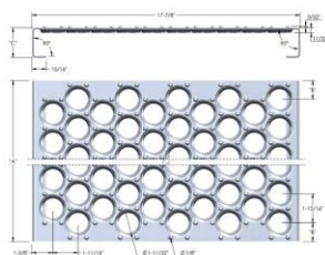
18" Width 10 Hole
