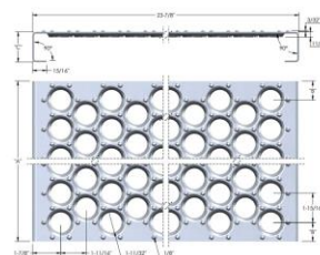
24" Width 13 Hole
