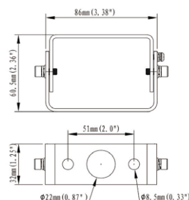
Yoke (30W/60W)
