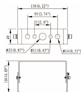
Yoke (100W/150W/200W/300W)
