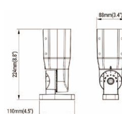
Ø76mm Slipfitter (100W/150W/200W/300W)
