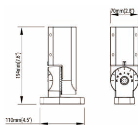
Ø60mm Slipfitter (100W/150W/200W/300W)
