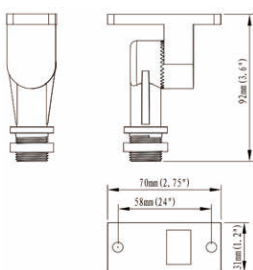
Knuckle (30W/60W)
