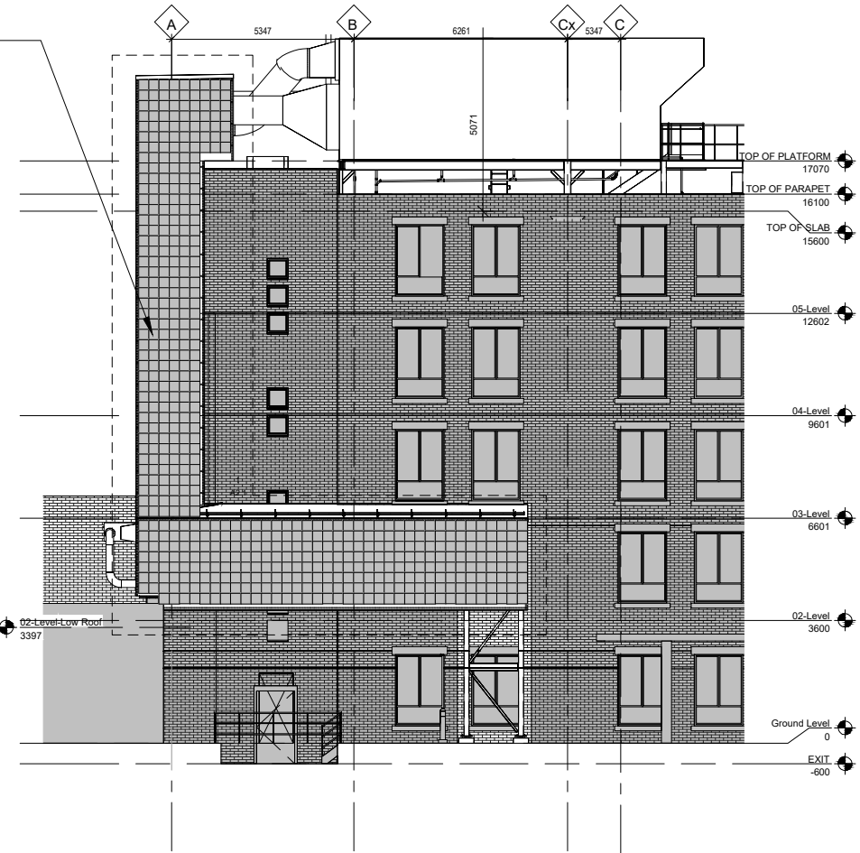
4 OVERALL WEST ELEVATION A1.1 PANELS SCALE : N/A
