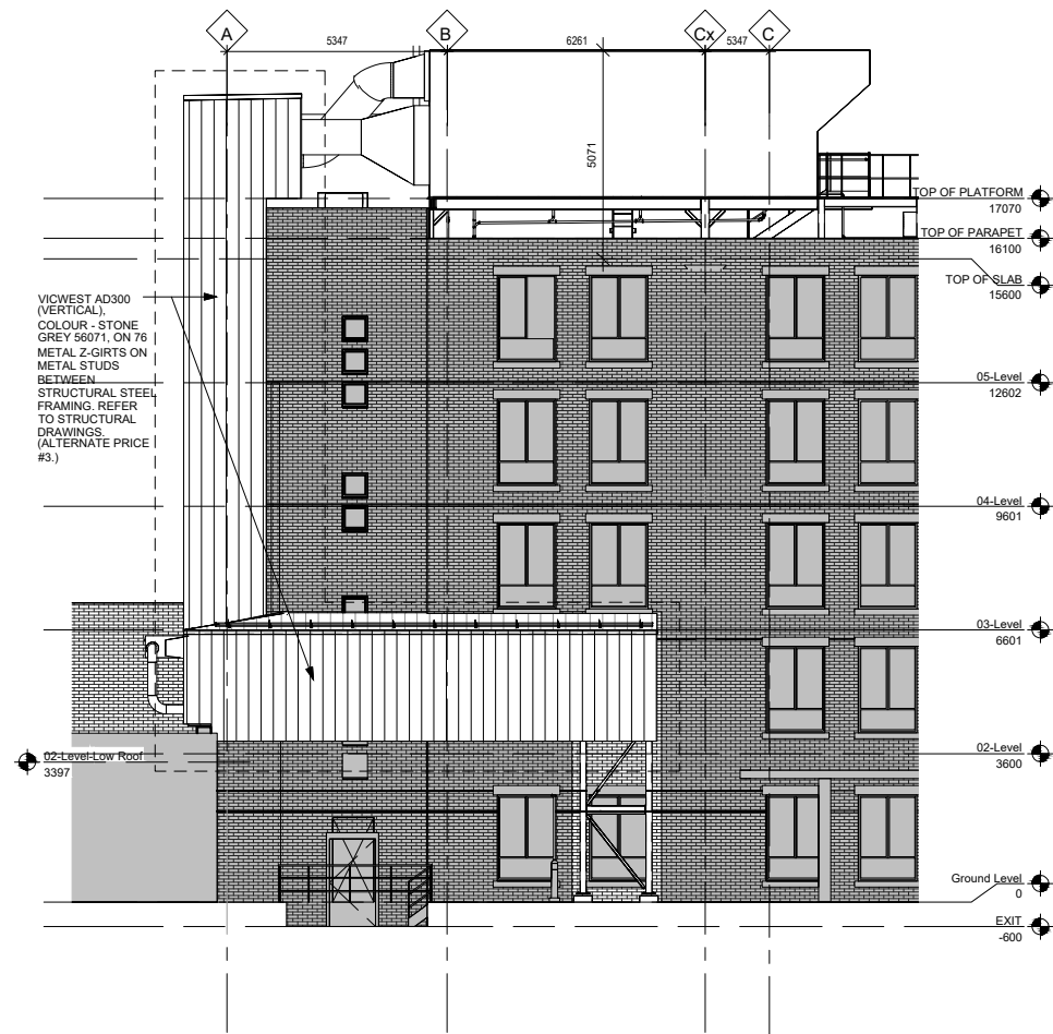
3 OVERALL WEST ELEVATION A1.0 SCALE : N/A
