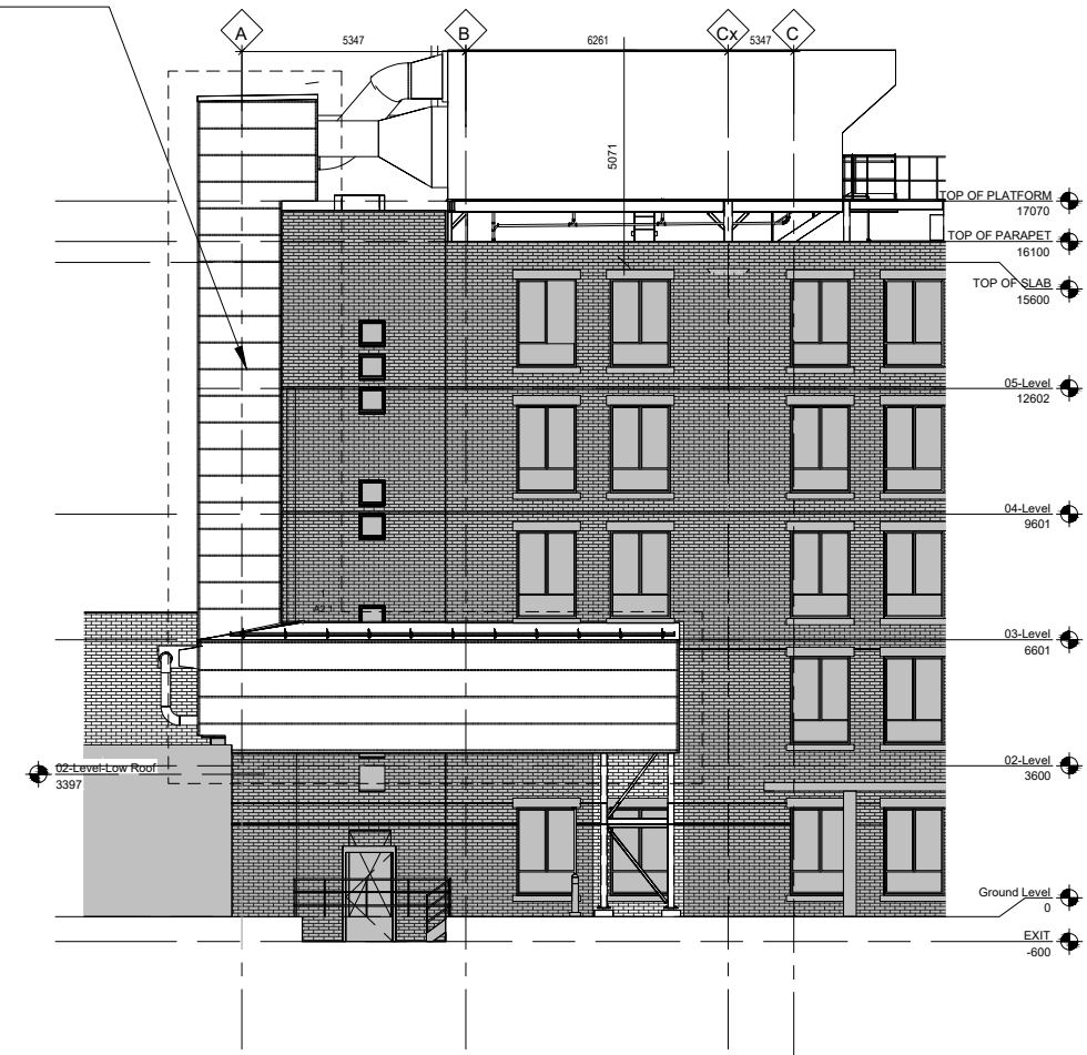
1 OVERALL WEST ELEVATION A1.1 SUB-Framing Behind Cladding SCALE : N/A
