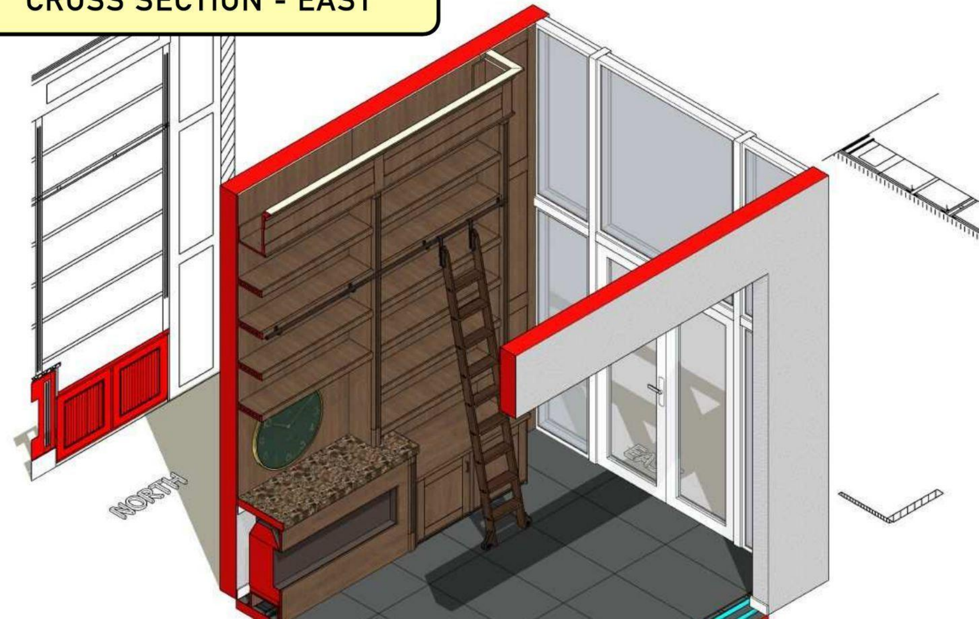
CROSS SECTION - EAST
