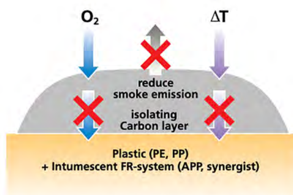
Figure 4: Mechanism of intumescent HFFR barrier layer
