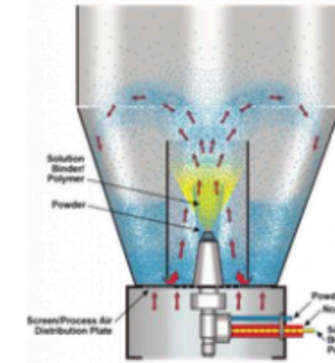
Processing Machine: Fluid Bed Coater for Coating by wurster COATING Technology Control: PLC 21 CFR Origin: India
