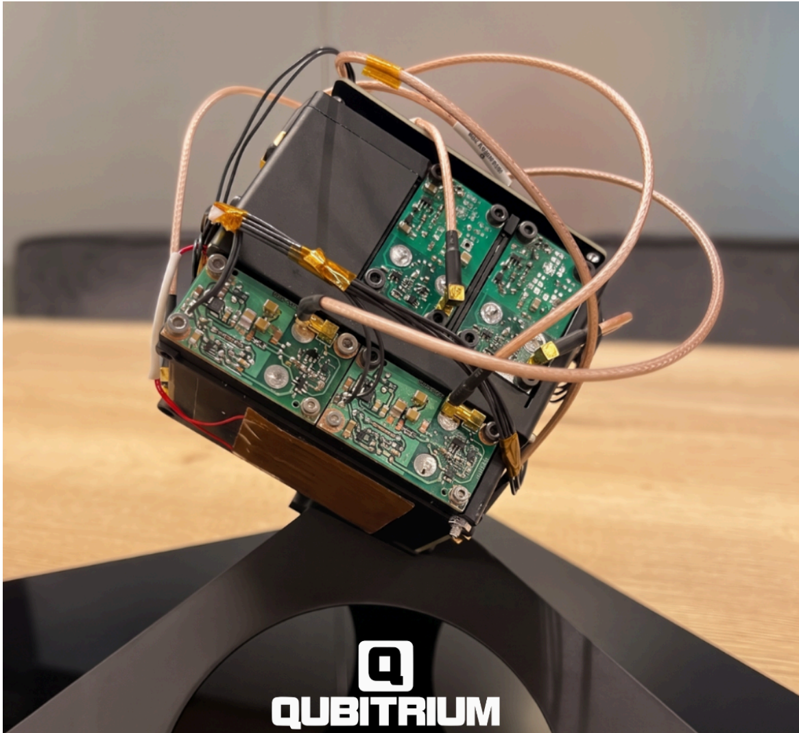
Figure 1: The QubitCore flight payload. A complete entanglement distribution system in 1U, 950 g. The boards on its faces are the single-photon detector channels; the coaxial cables carry their output pulses to the time tagger.
