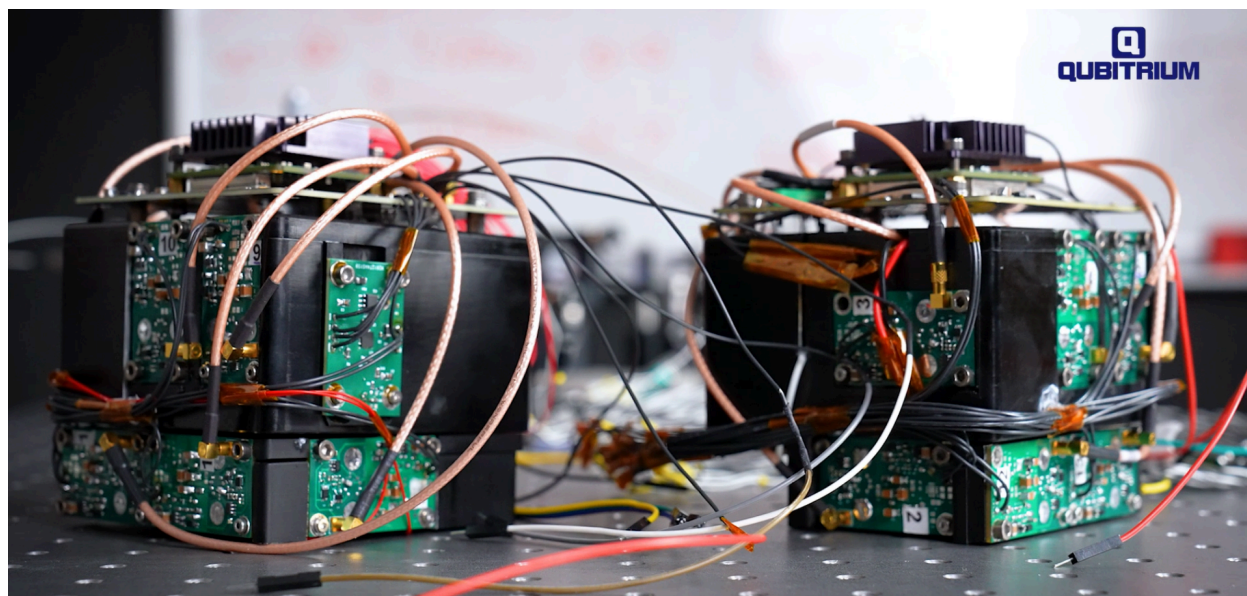
Figure 5: The first prototypes of QubitCore on the optical bench.
