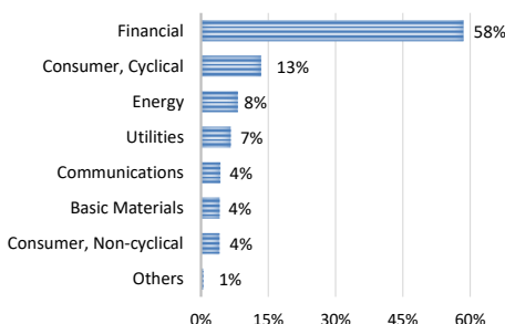
SECTORAL EXPOSURE 4
