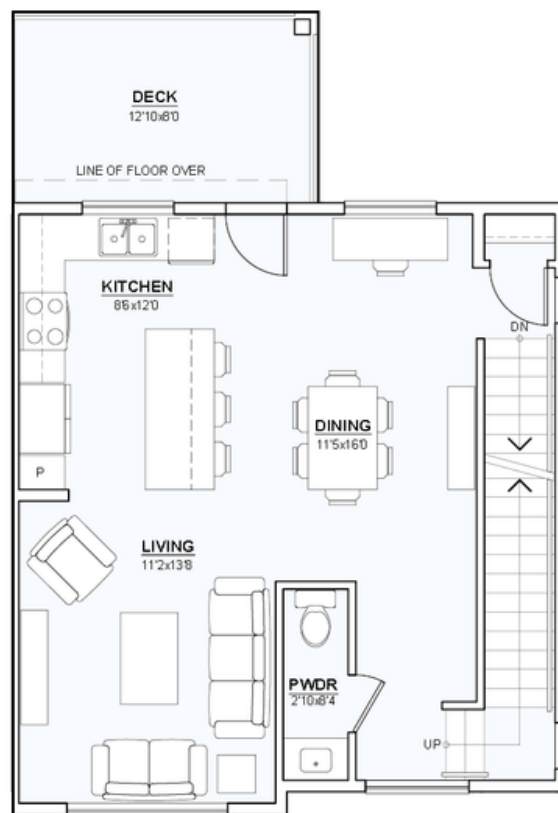
MAIN FLOOR PLAN AREA: 632 sf.
