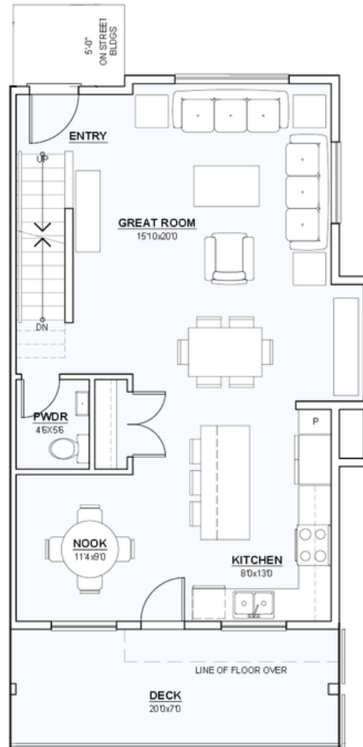
MAIN FLOOR PLAN AREA: 704 sf
