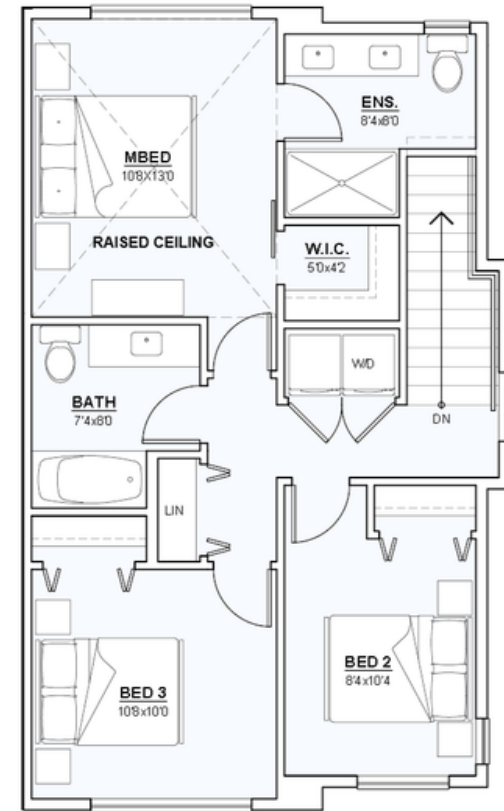
UPPER FLOOR PLAN AREA : 704 sf
