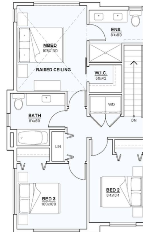
UPPER FLOOR PLAN AREA : 703 sf
