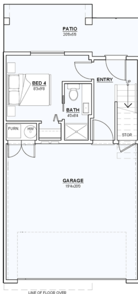
LOWER FLOOR PLAN AREA : 265 sf GARAGE AREA : 410 sf
