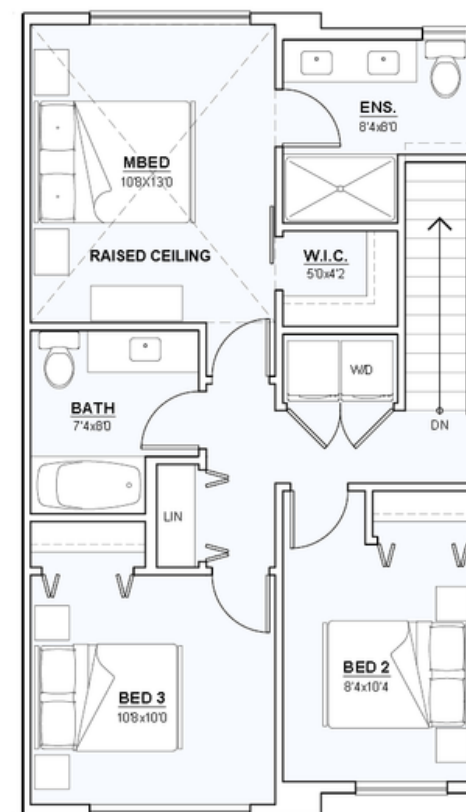
UPPER FLOOR PLAN AREA : 688 sf
