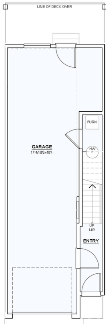
LOWER FLOOR PLAN AREA: 110 sf. GARAGE AREA: 499 sf.
