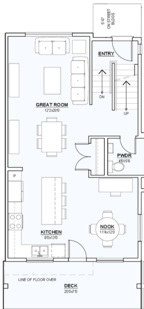
MAIN FLOOR PLAN AREA: 690 sf
