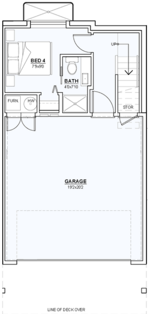
LOWER FLOOR PLAN AREA: 264 sf GARAGE AREA: 417 sf
