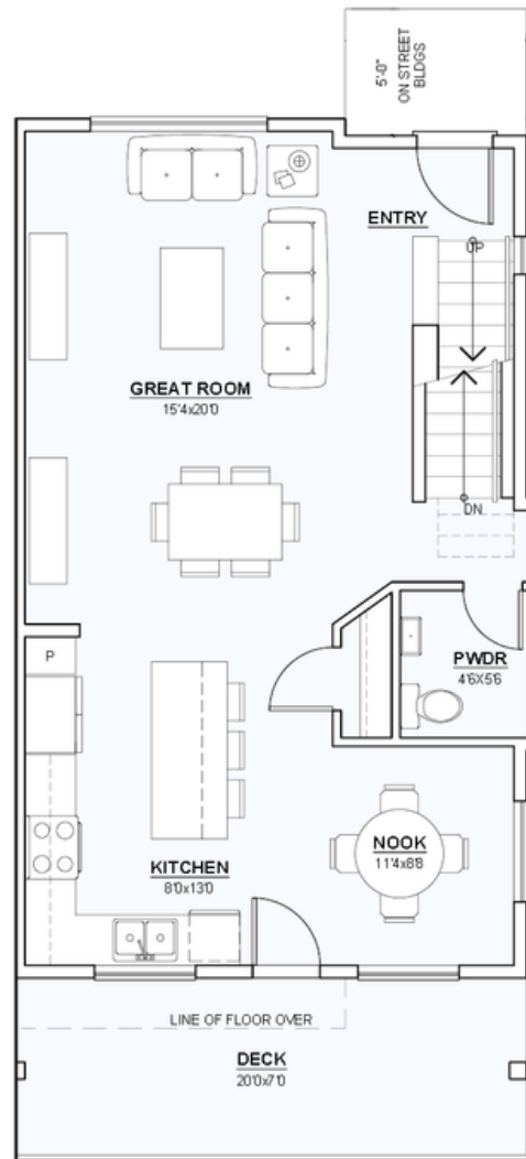
MAIN FLOOR PLAN AREA: 688 sf
