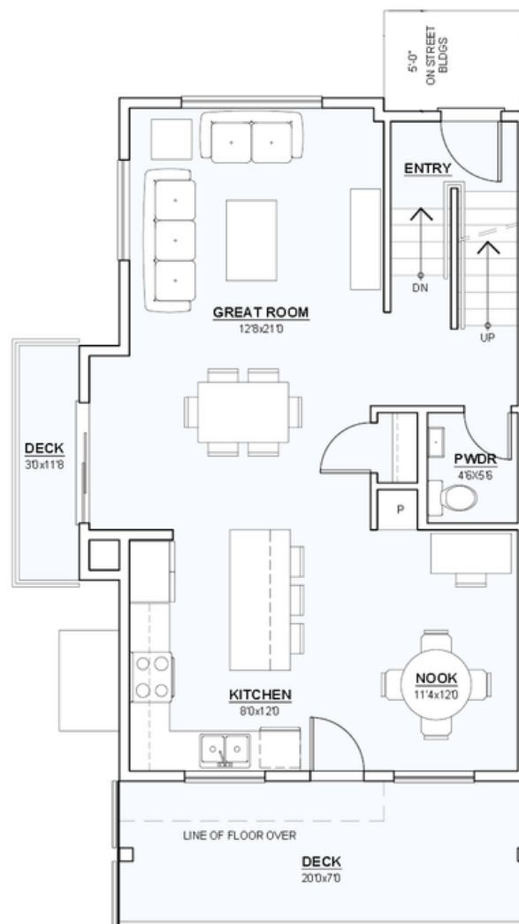
MAIN FLOOR PLAN AREA: 704 sf
