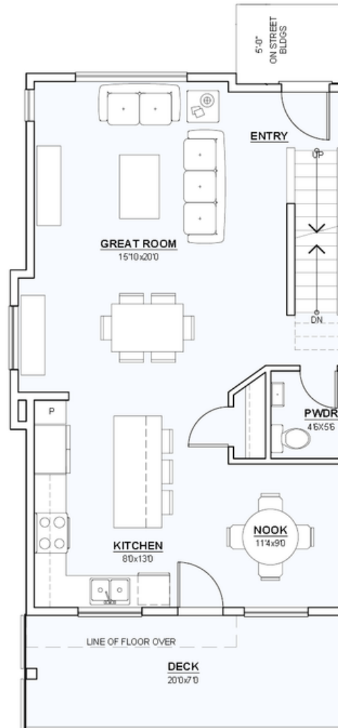
MAIN FLOOR PLAN AREA: 691 sf
