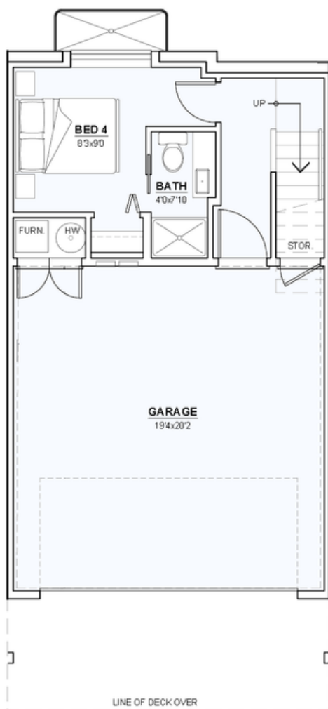
LOWER FLOOR PLAN AREA: 262 sf GARAGE AREA: 413 sf
