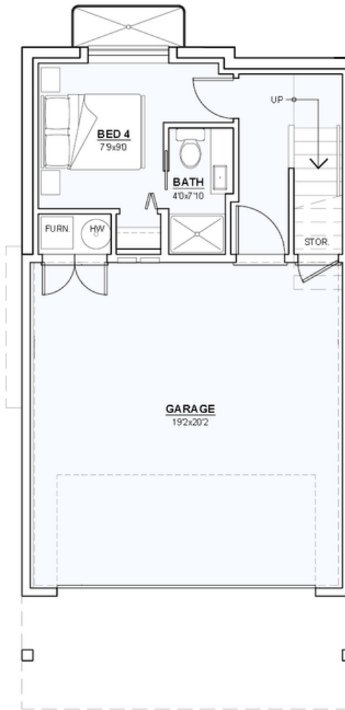
LOWER FLOOR PLAN AREA: 264 sf GARAGE AREA: 417 sf
