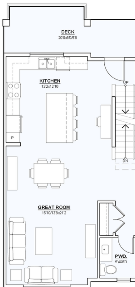
MAIN FLOOR PLAN AREA : 688 sf
