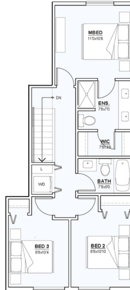
UPPER FLOOR PLAN AREA: 627 sf.
