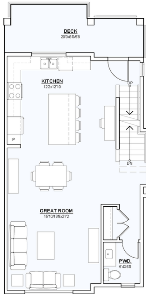
MAIN FLOOR PLAN AREA : 704 sf
