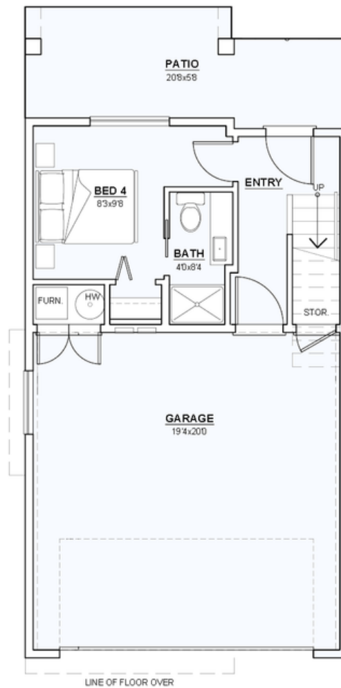
LOWER FLOOR PLAN AREA : 268 sf GARAGE AREA : 413 sf
