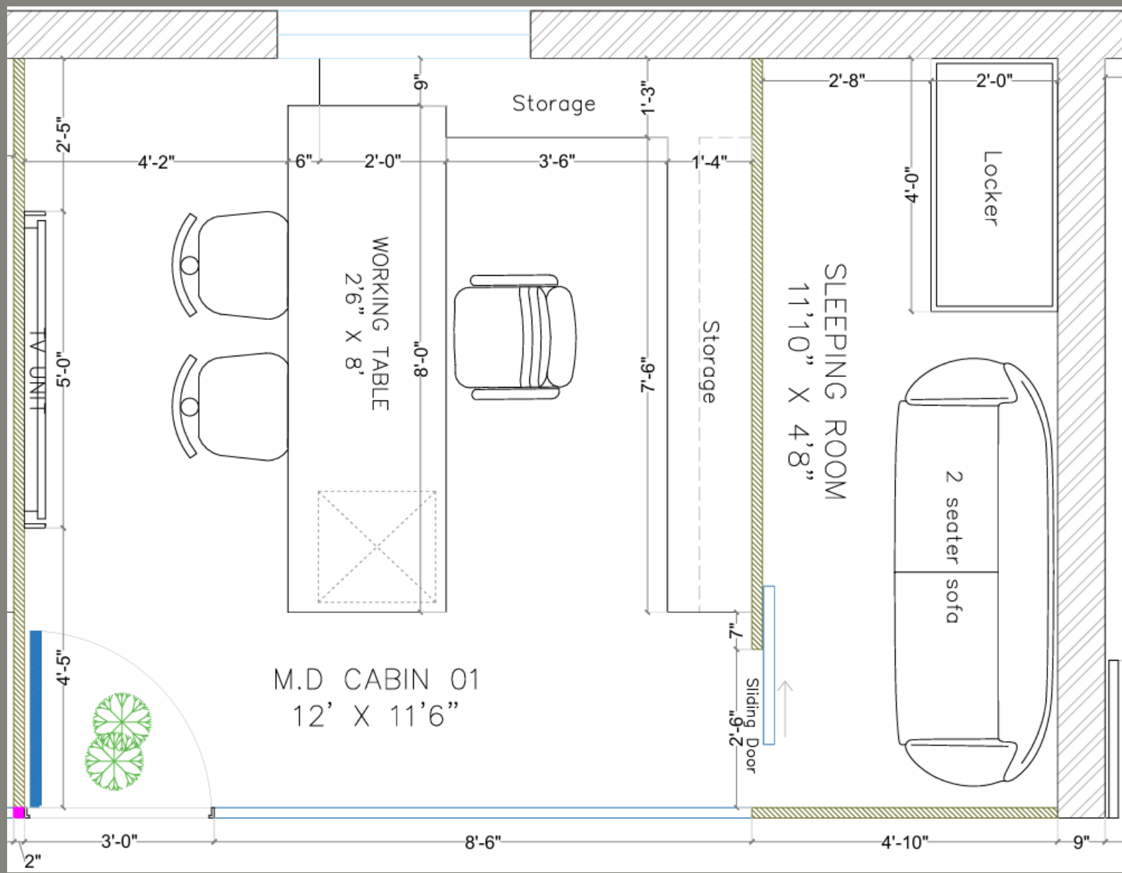
PLAN
