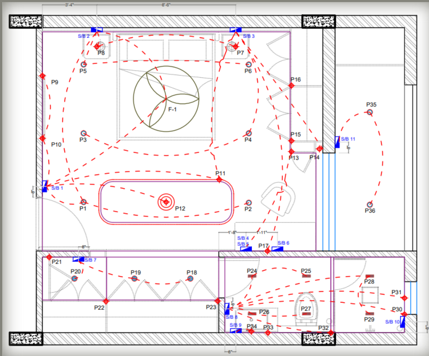
ELECTRICAL LOOPING LAYOUT
