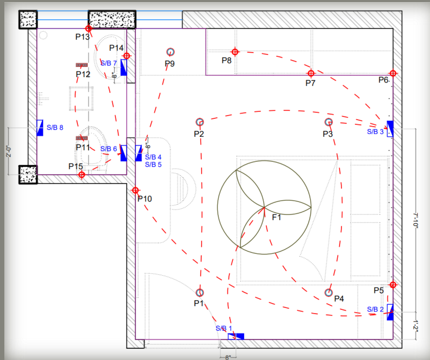
ELECTRICAL LOOPING LAYOUT
