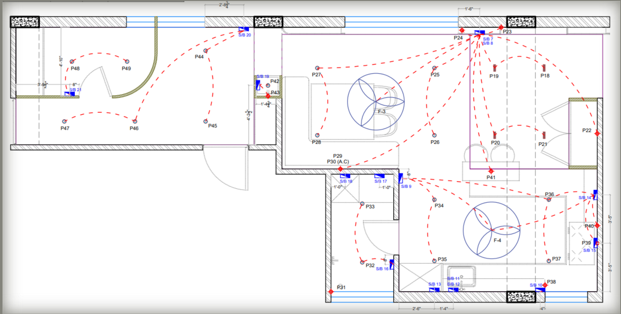
ELECTRICAL LOOPING LAYOUT
