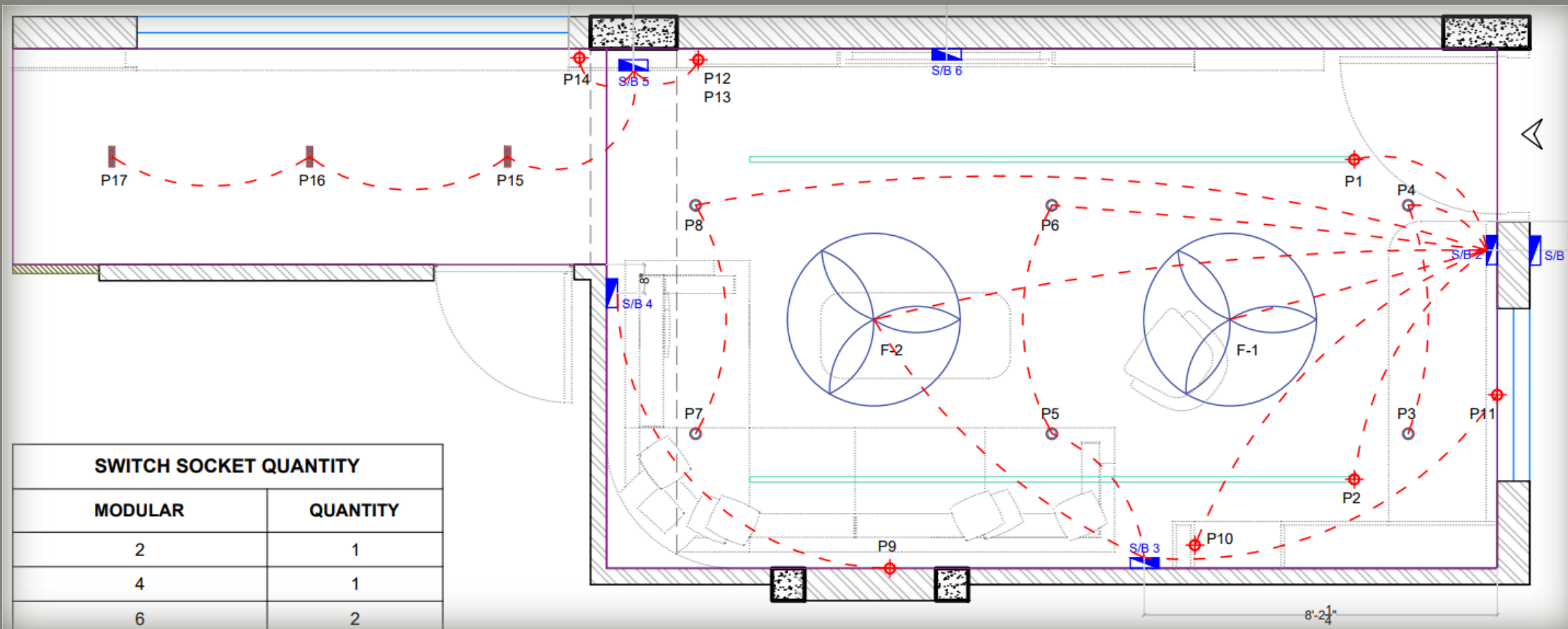
ELECTRICAL LOOPING LAYOUT
