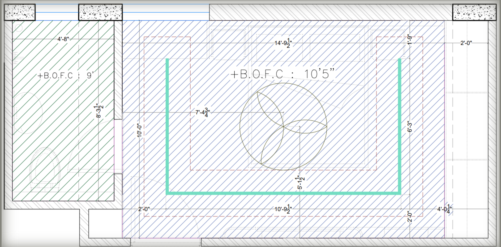
CEILING LAYOUT
