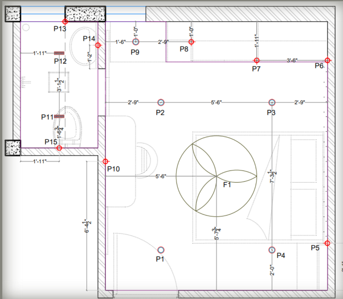
ELECTRICAL LAYOUT
