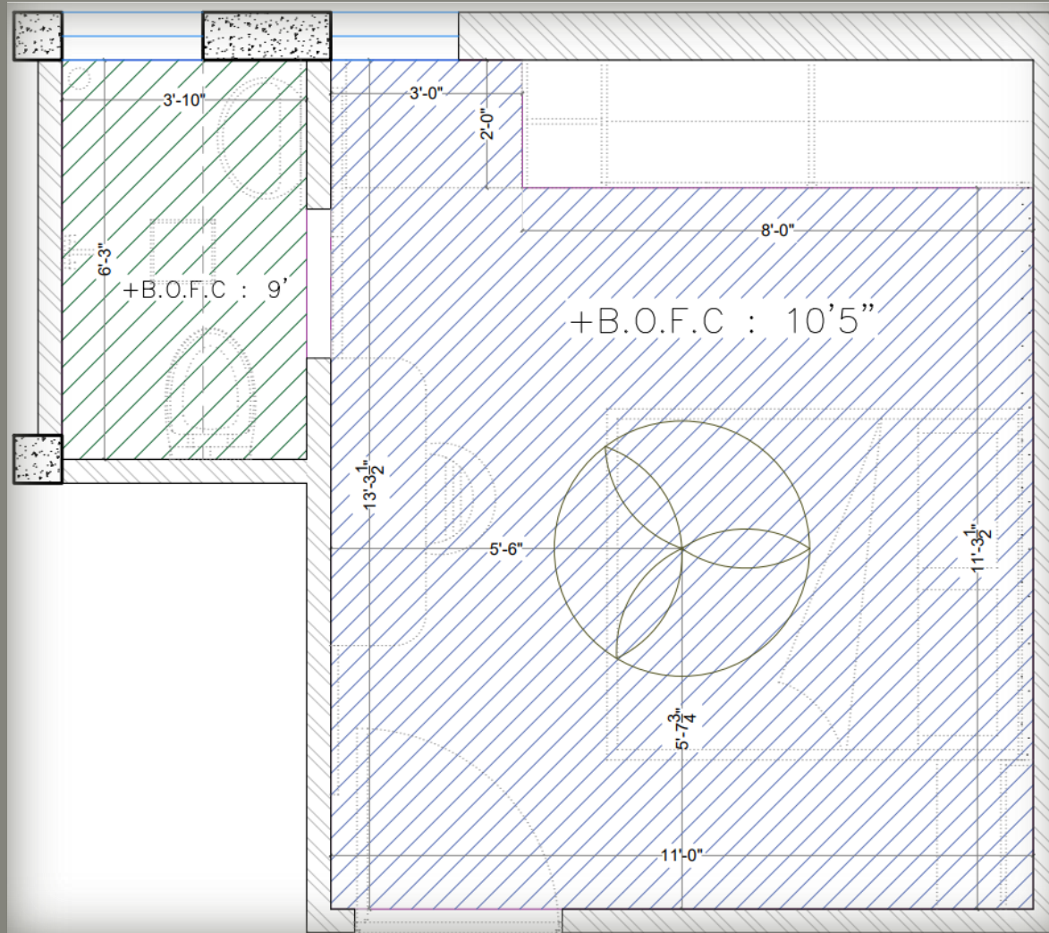
CEILING LAYOUT
