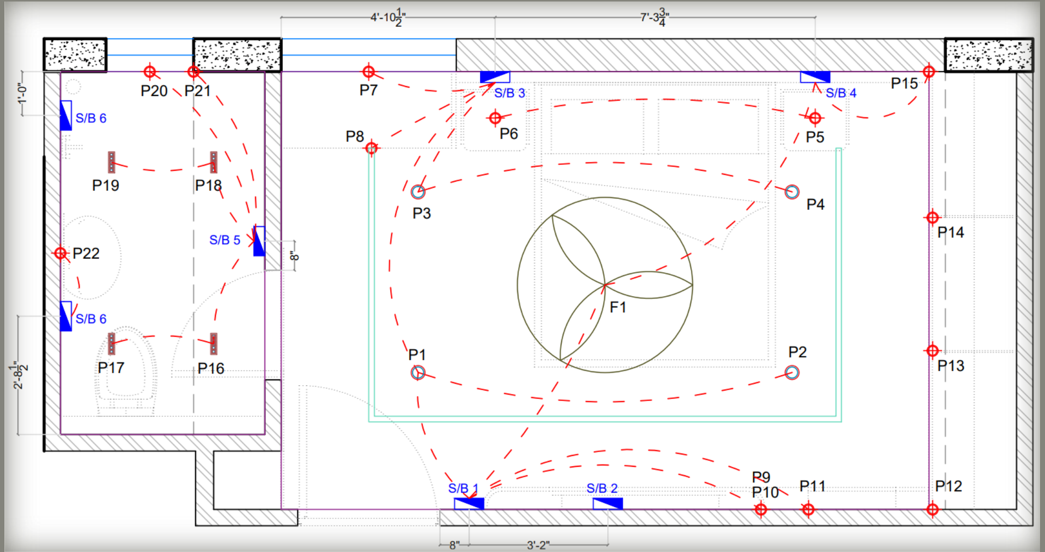
ELECTRICAL LOOPING LAYOUT
