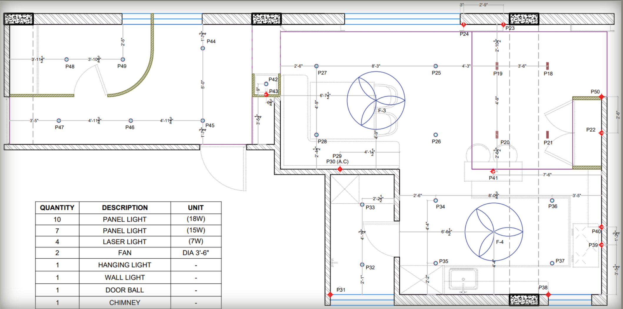
ELECTRICAL LAYOUT
