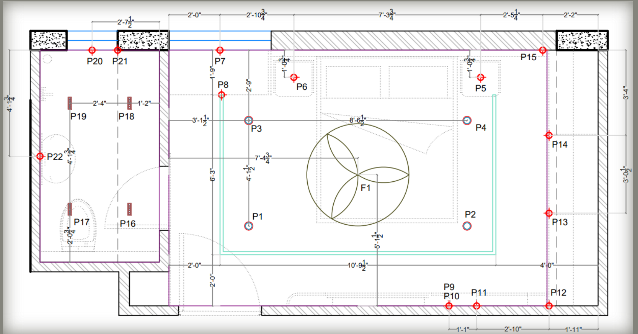
ELECTRICAL LAYOUT
