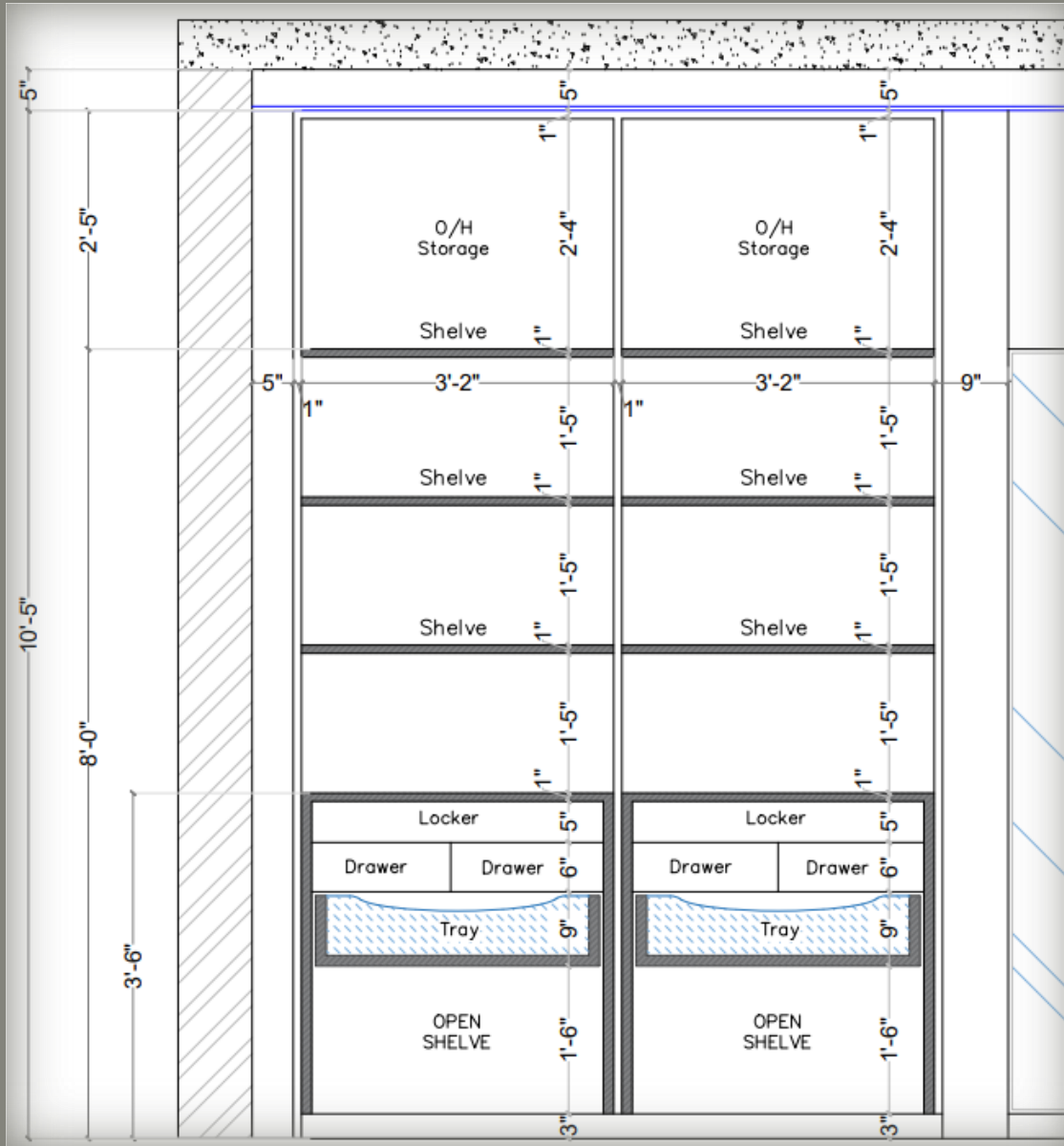
WARDROBE INTERNAL
