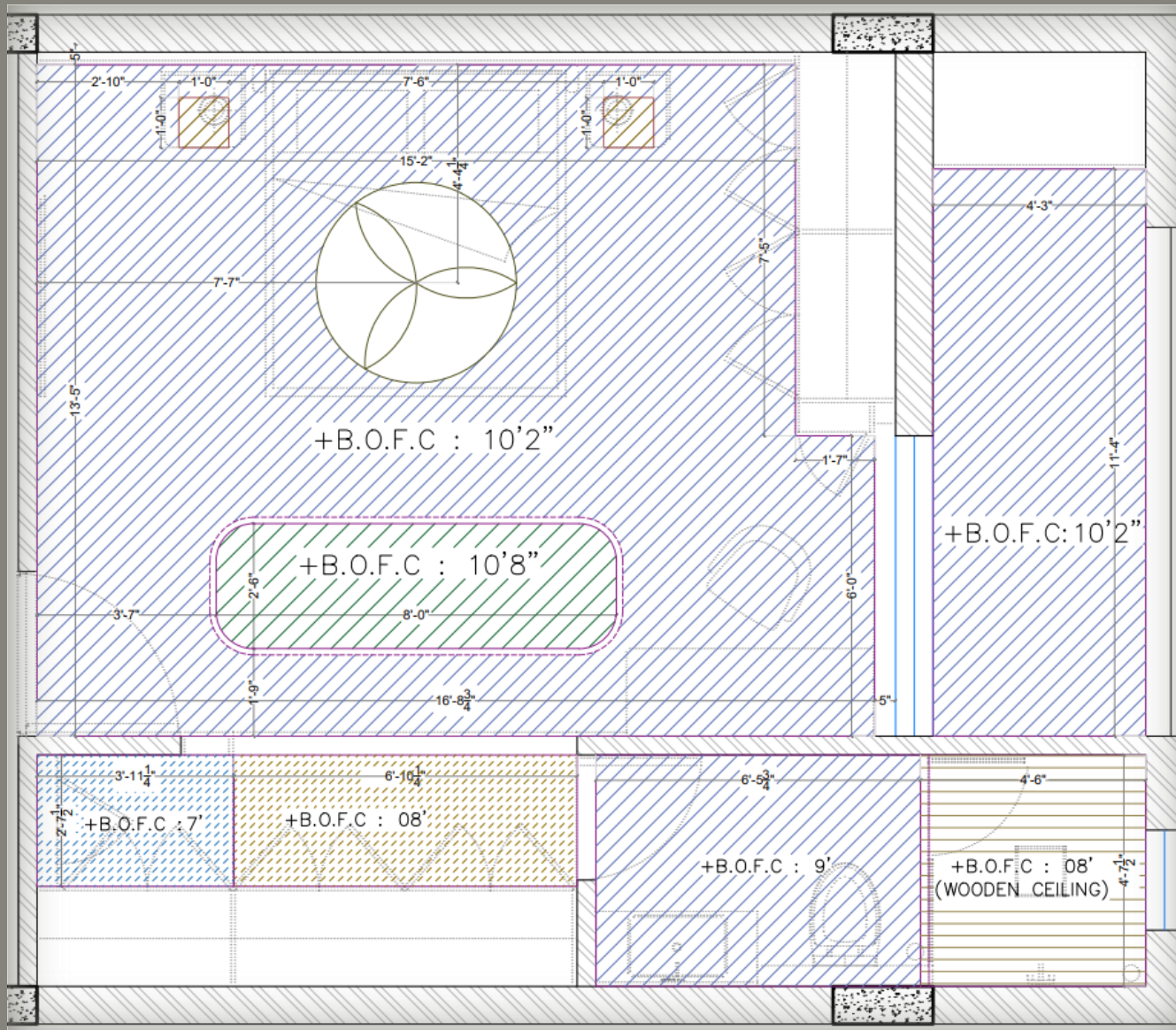
CEILING LAYOUT
