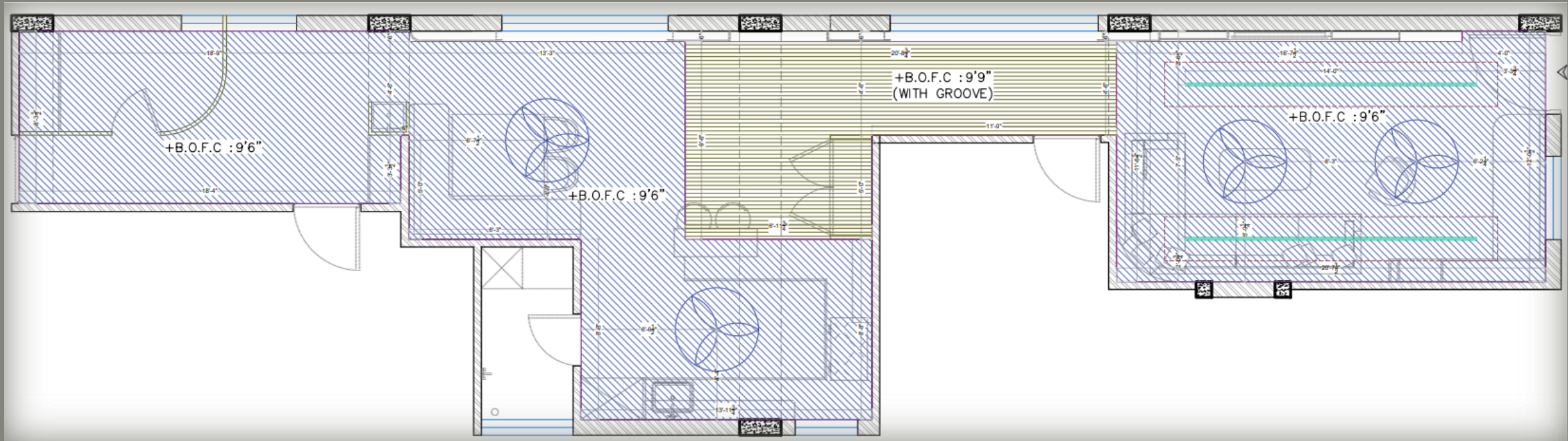
CEILING LAYOUT
