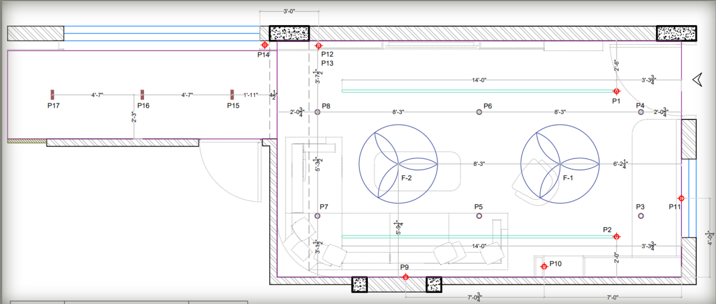
ELECTRICAL LAYOUT
