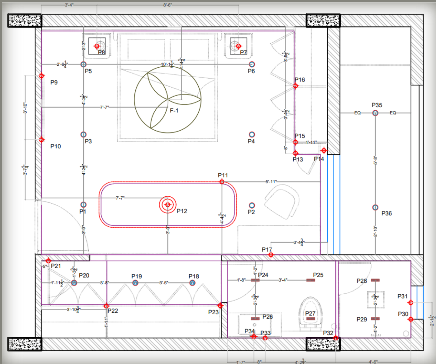
ELECTRICAL LAYOUT
