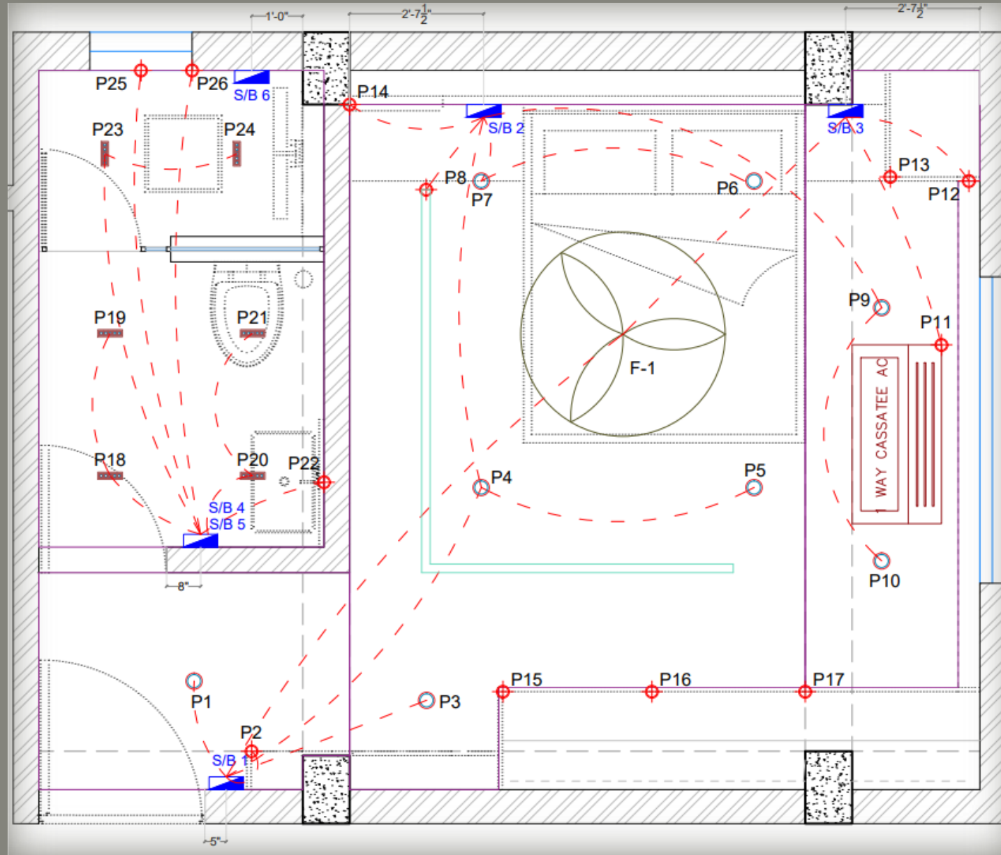
ELECTRICAL LOOPING LAYOUT
