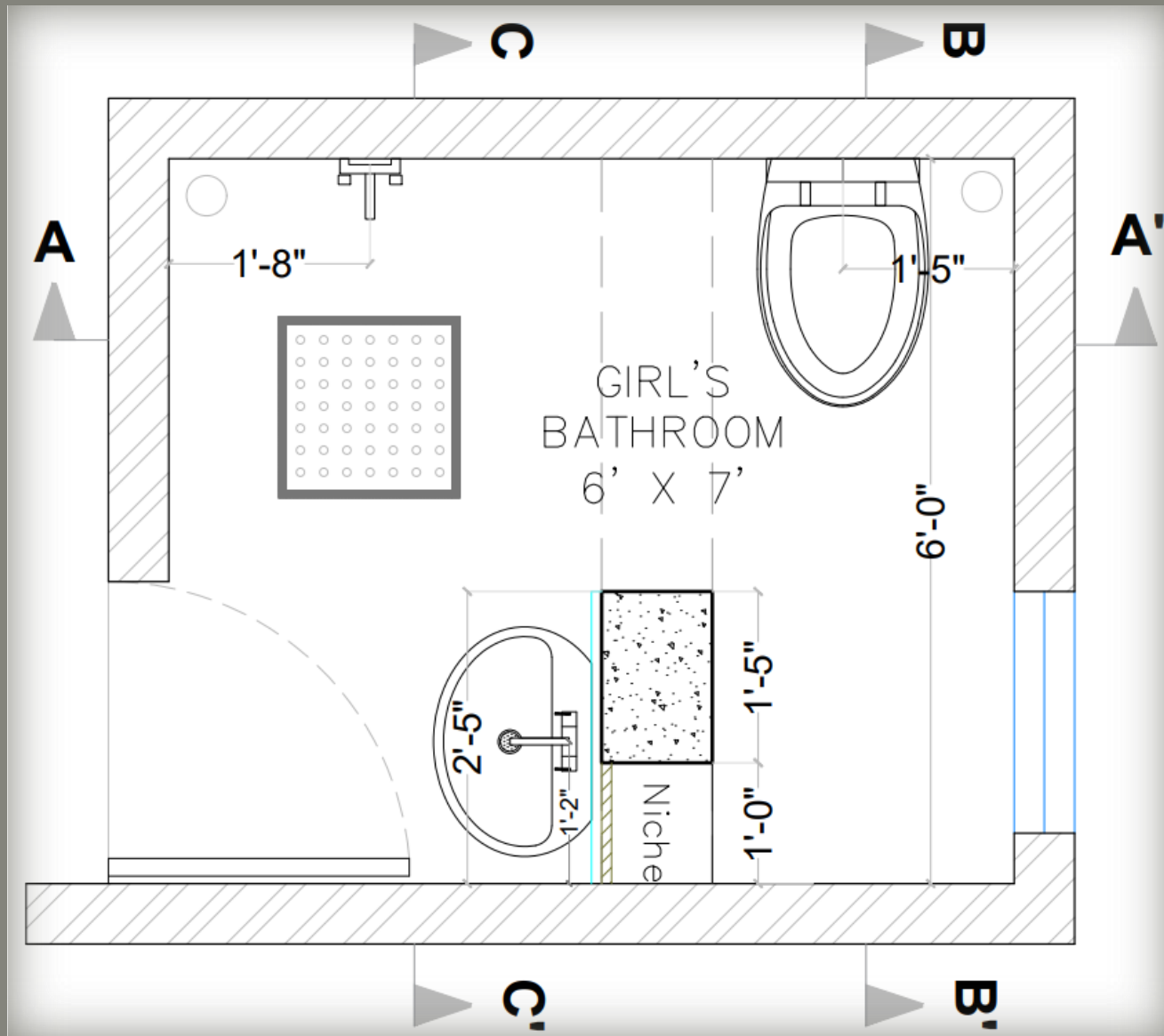
BATHROOM LAYOUT
