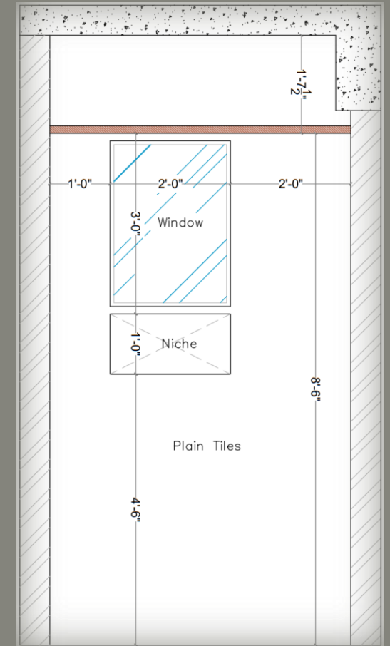
ELEVATION-CC'
