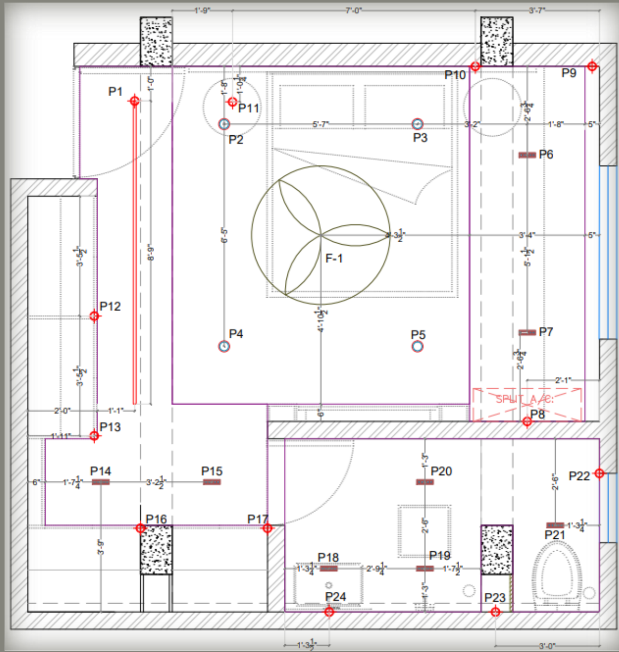
ELECTRICAL LAYOUT
