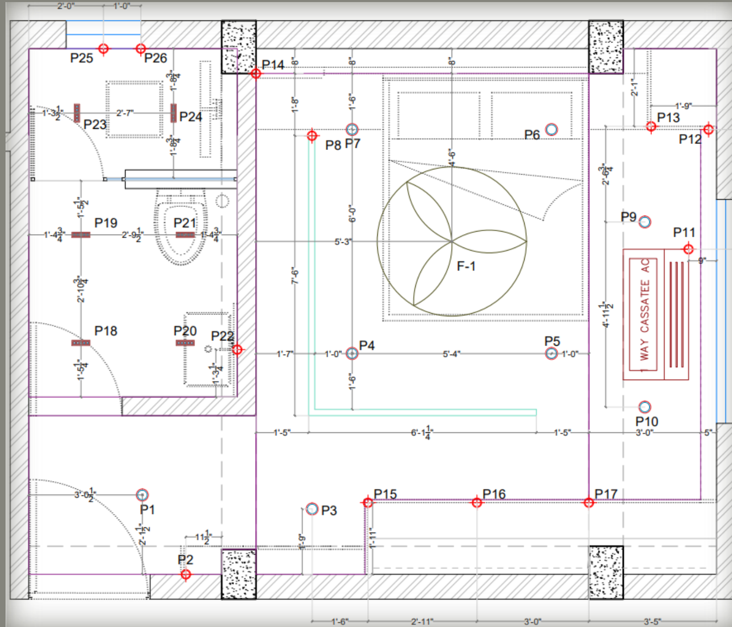
ELECTRICAL LAYOUT
