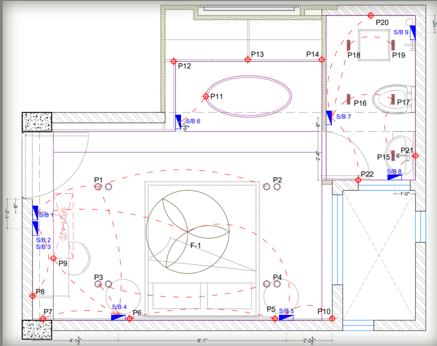
ELECTRICAL LOOPING LAYOUT
