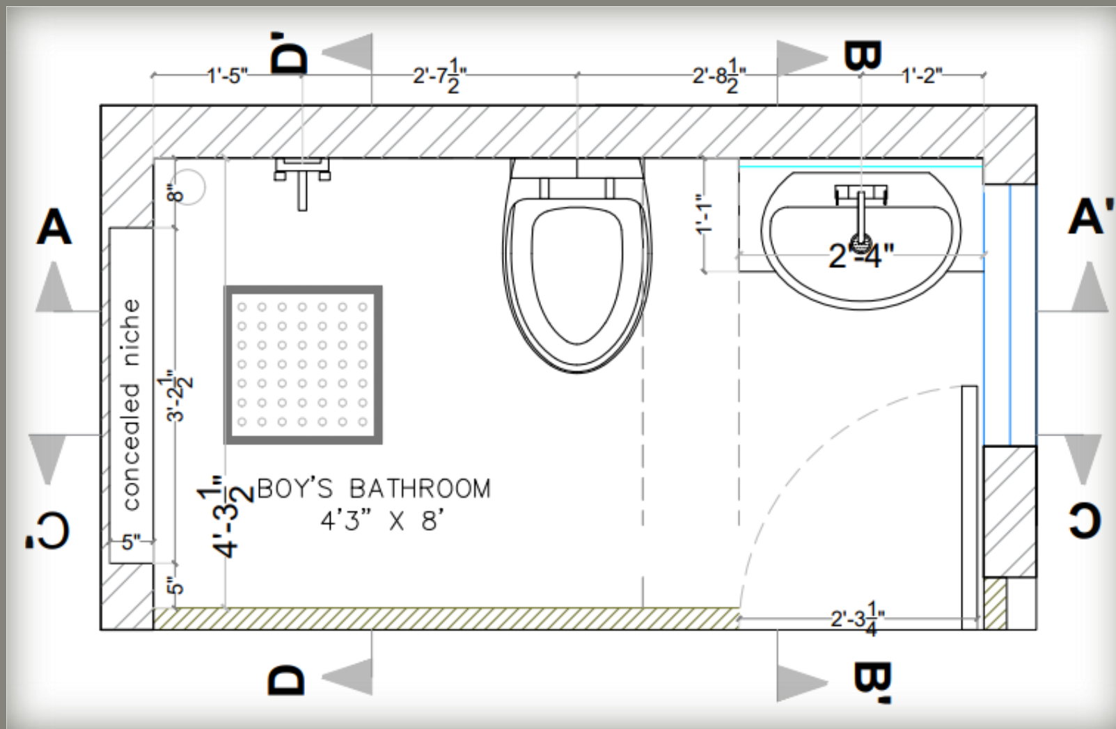
BATHROOM LAYOUT
