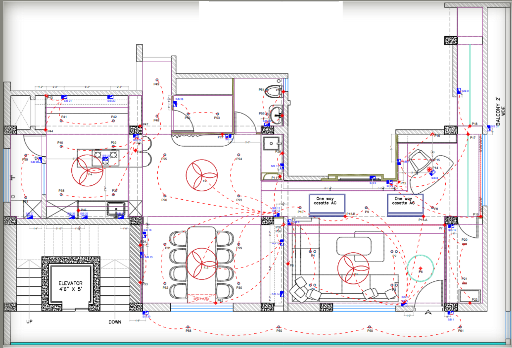
ELECTRICAL LOOPING LAYOUT
