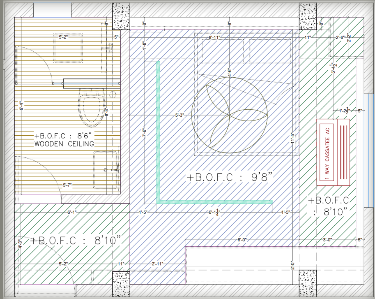
CEILING LAYOUT
