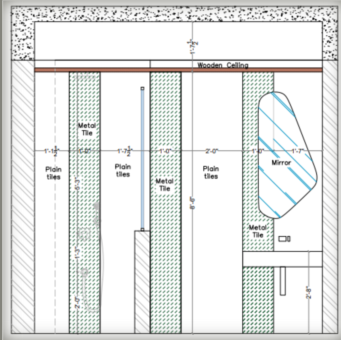
ELEVATION-AA'
