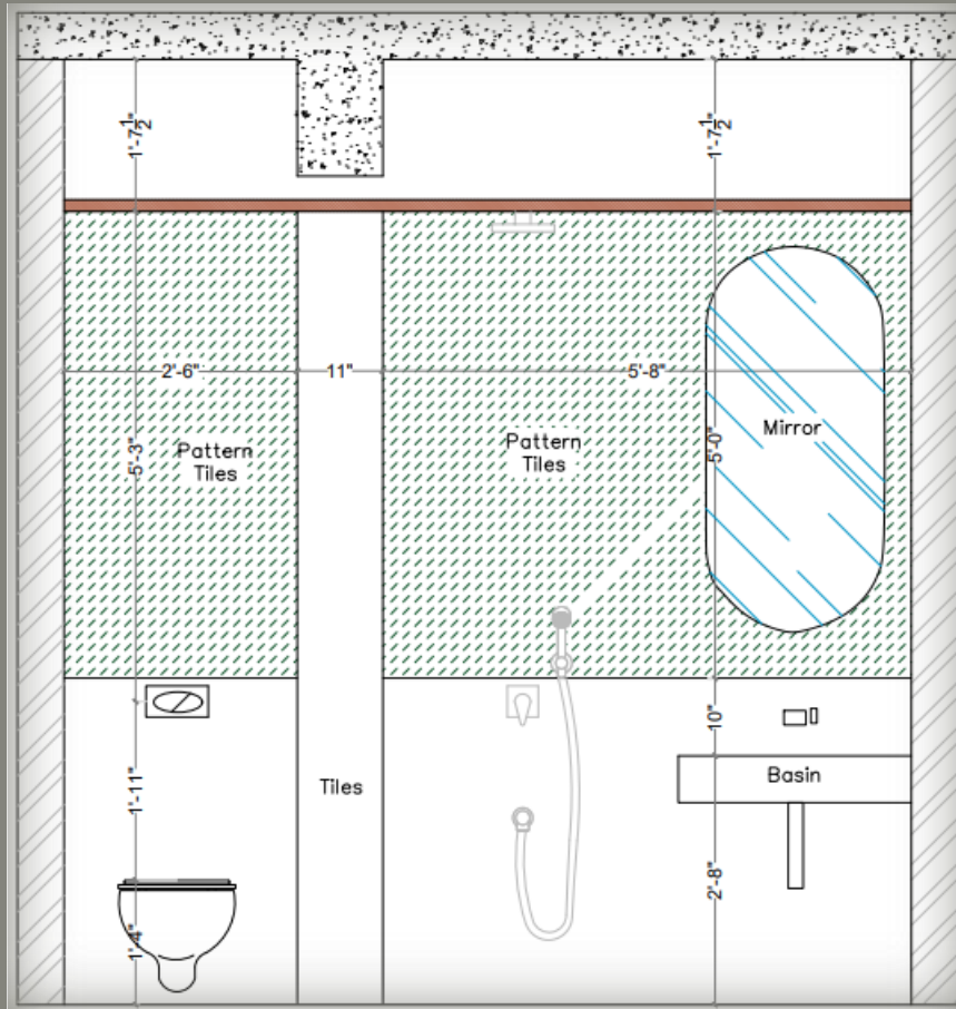
ELEVATION-AA'
