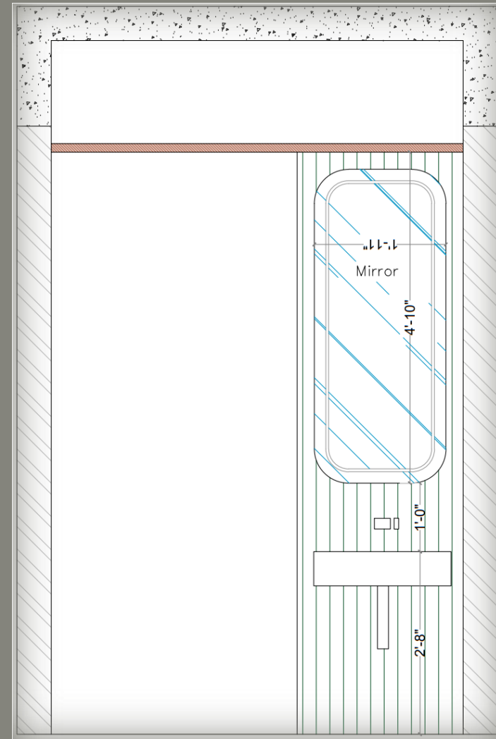
ELEVATION-CC'
