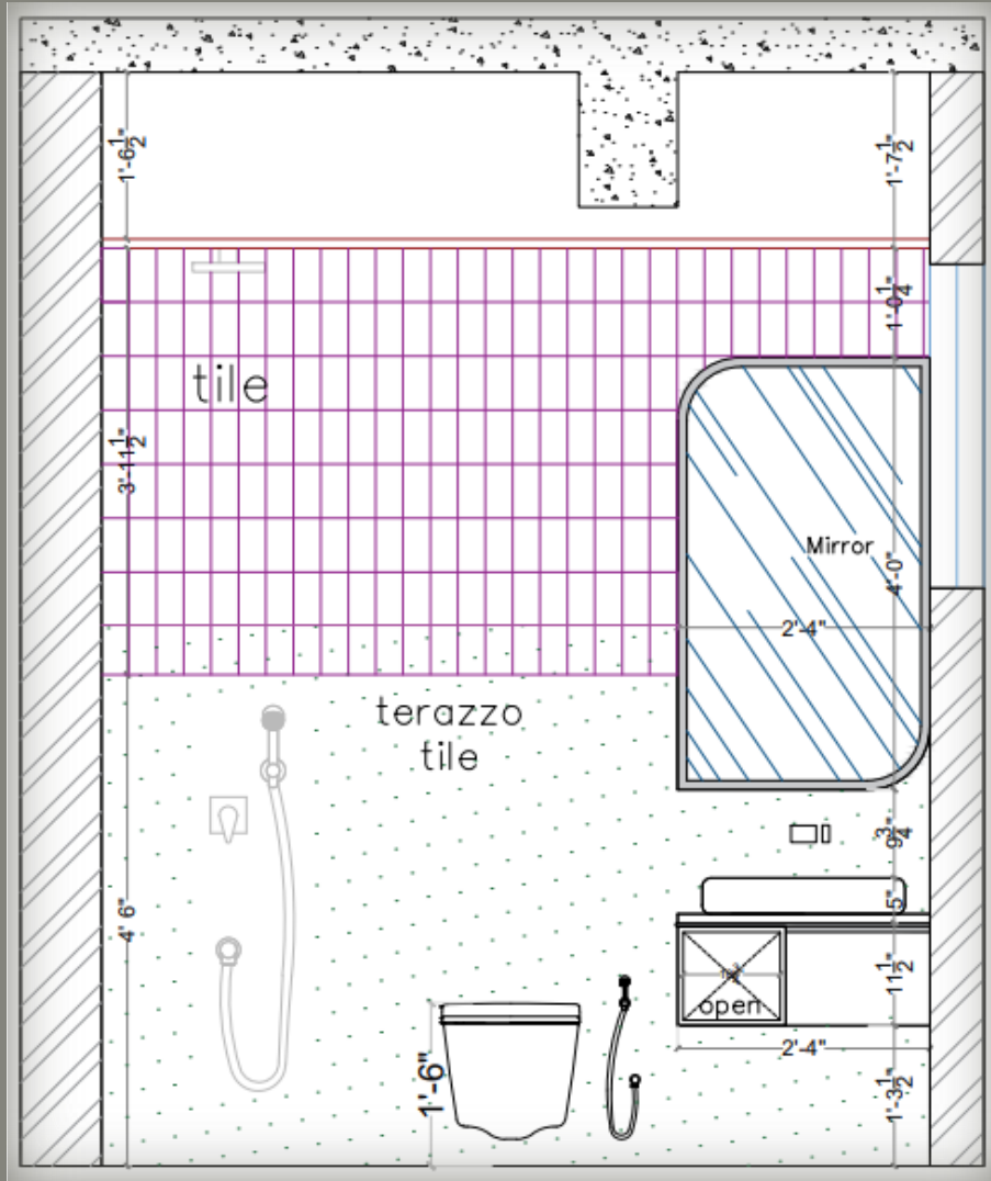
ELEVATION-AA'
