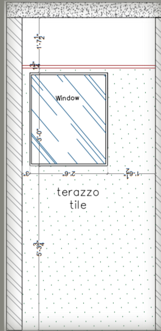
ELEVATION-BB'
