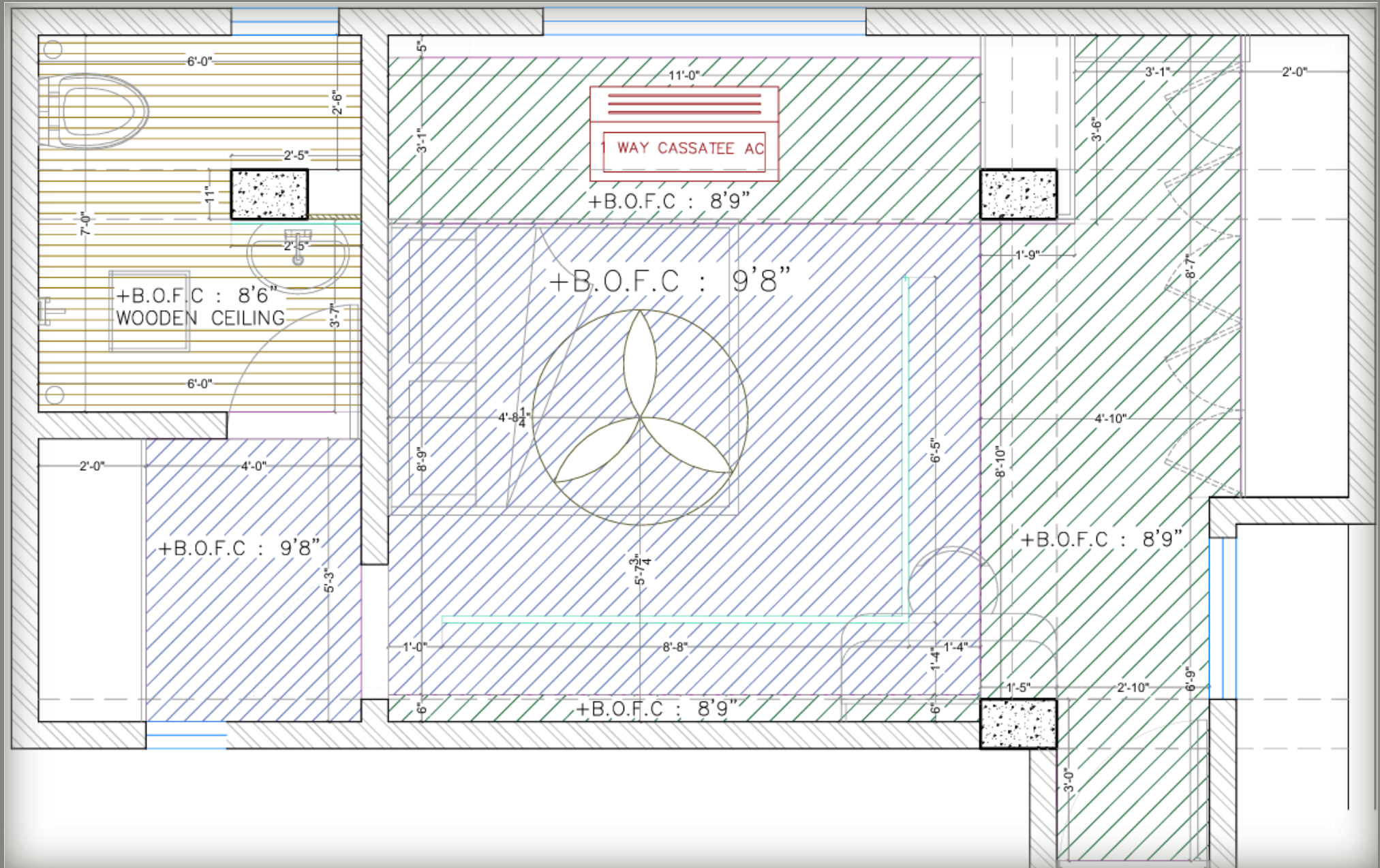
CEILING LAYOUT
