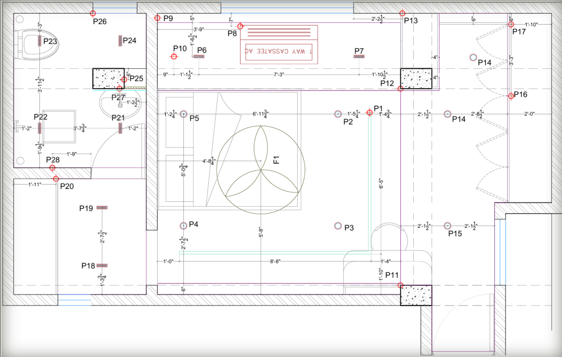
ELECTRICAL LAYOUT
