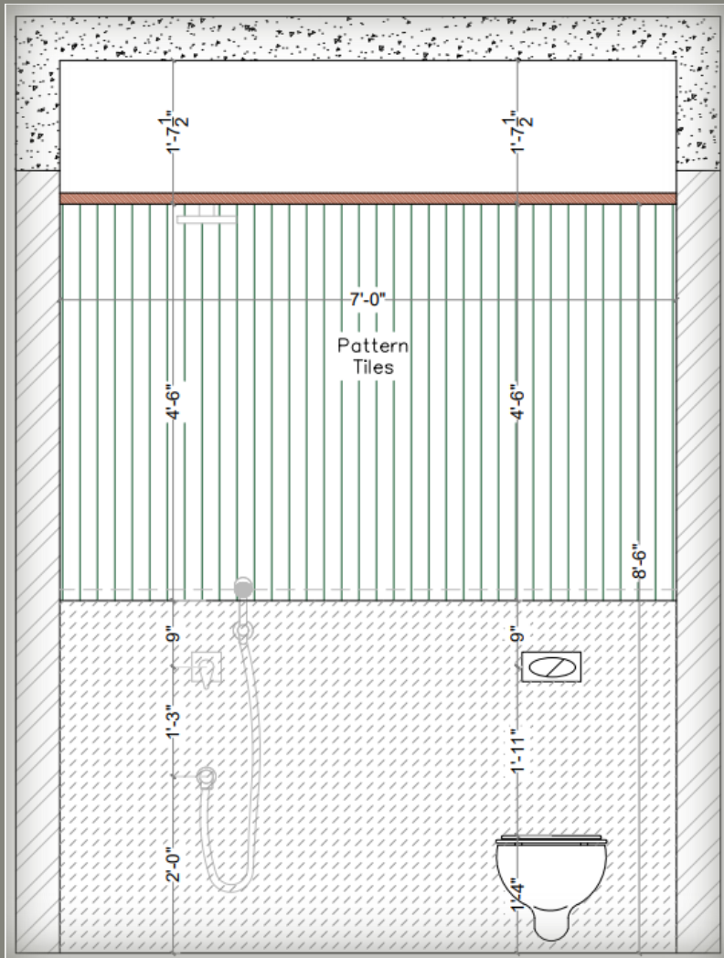
ELEVATION-AA'
