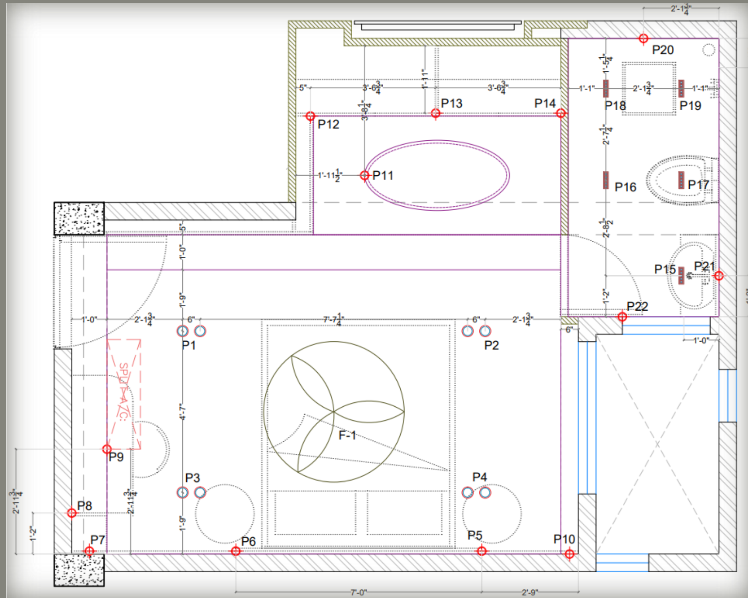
ELECTRICAL LAYOUT
