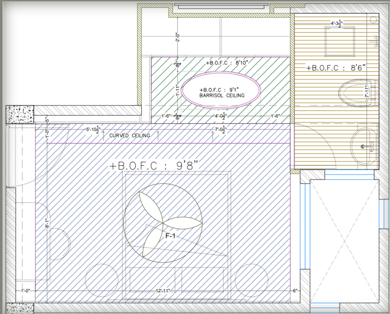
CEILING LAYOUT
