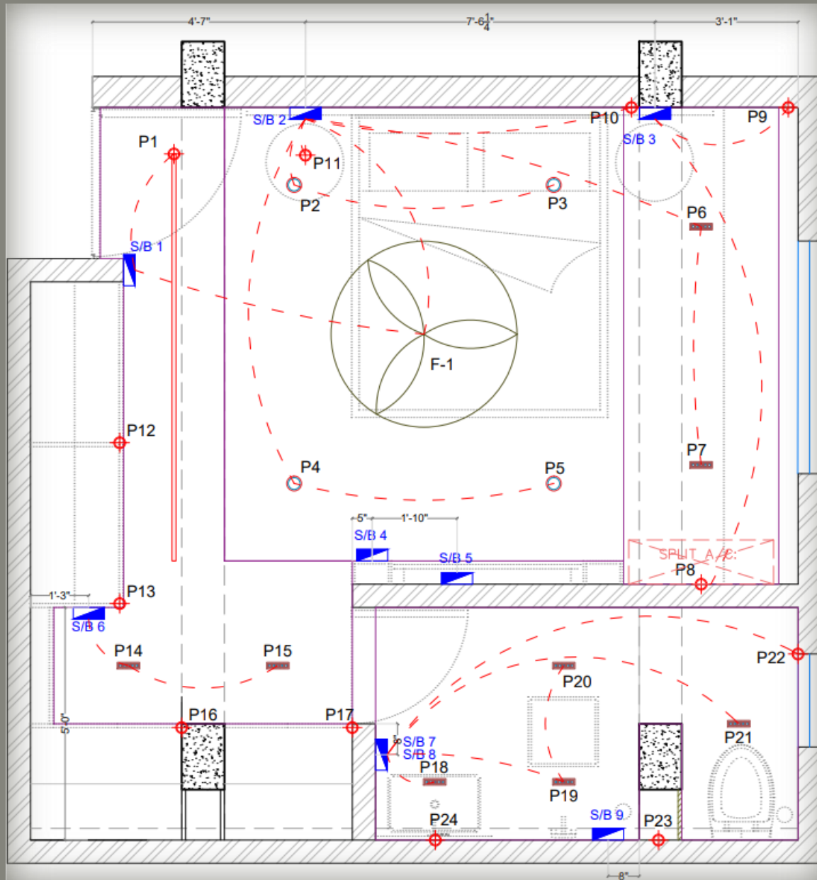
ELECTRICAL LOOPING LAYOUT
