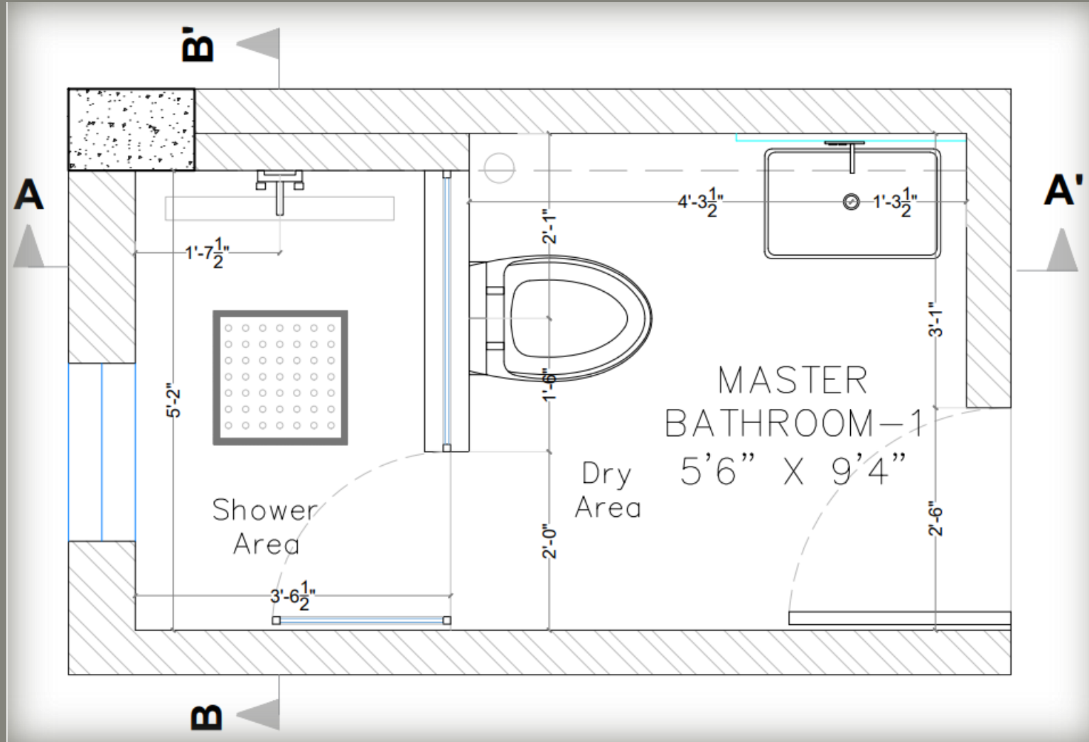
BATHROOM LAYOUT
