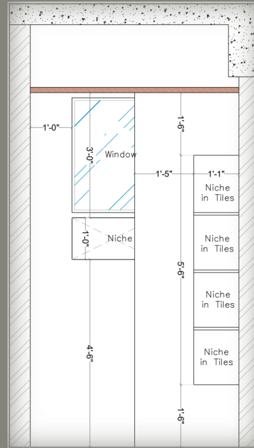
ELEVATION-BB'
