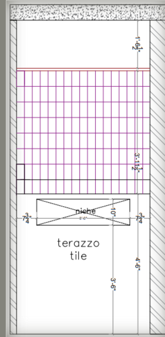
ELEVATION-BB'
