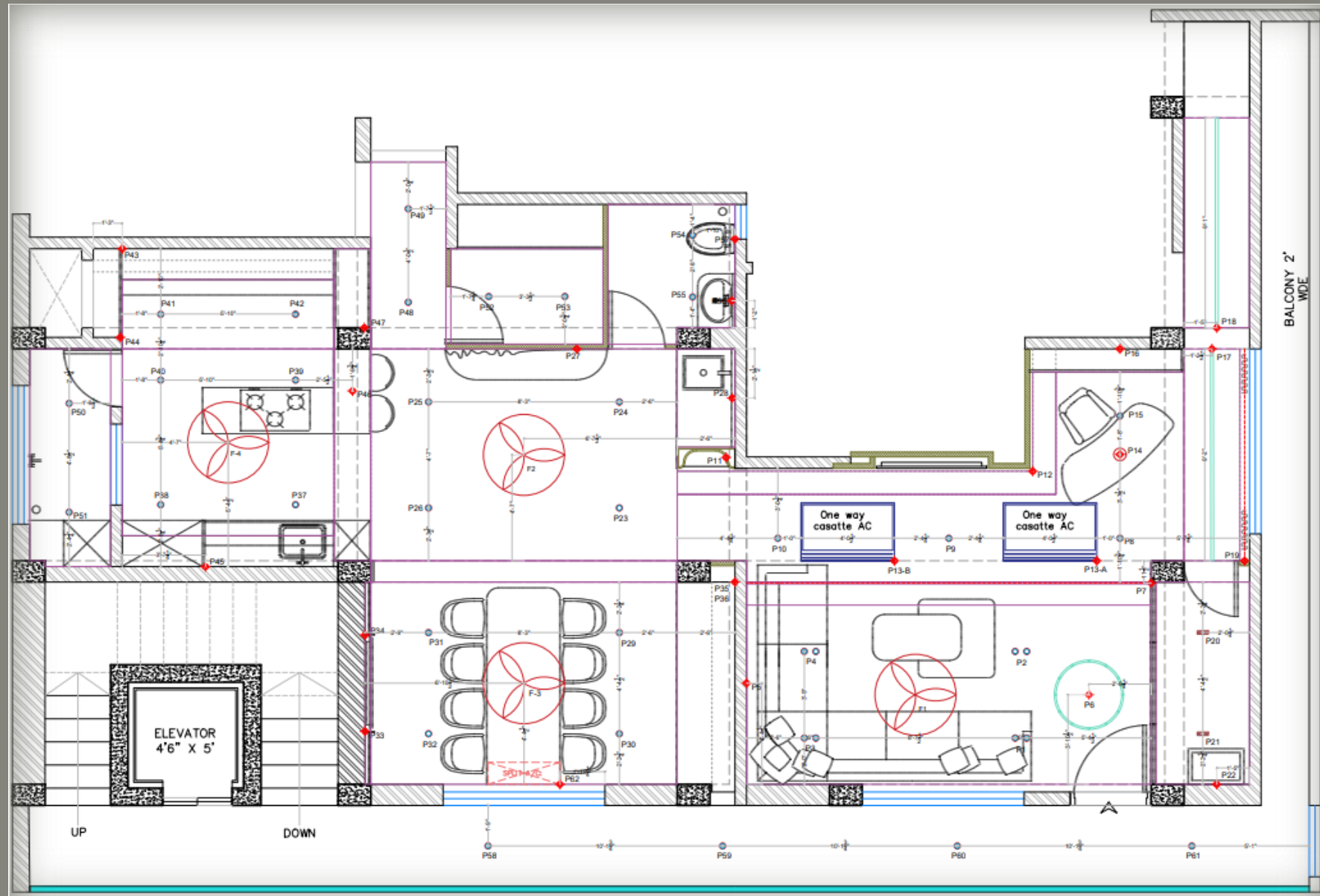
ELECTRICAL LAYOUT
