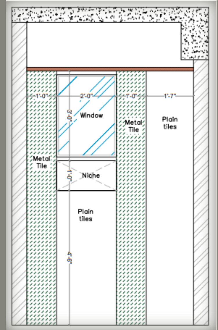
ELEVATION-BB'
