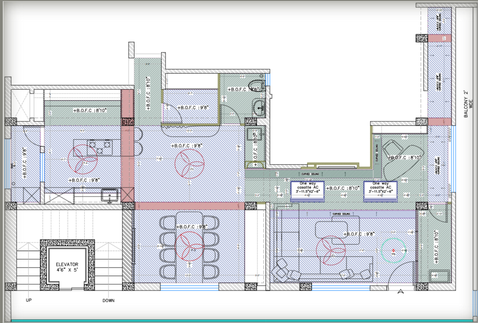
CEILING LAYOUT
