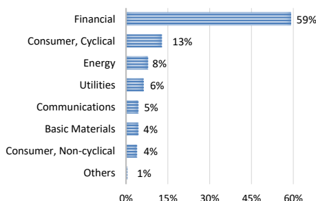
SECTORAL EXPOSURE 4
