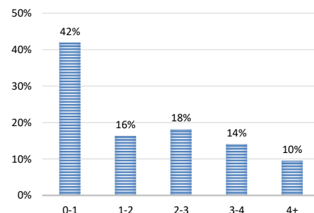
PORTFOLIO DURATION 2
