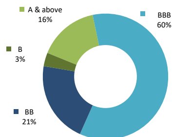
RATING PROFILE 1
