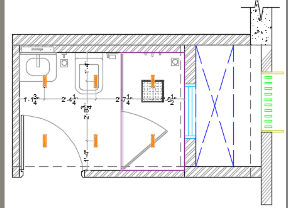
ELECTRICAL PLAN
