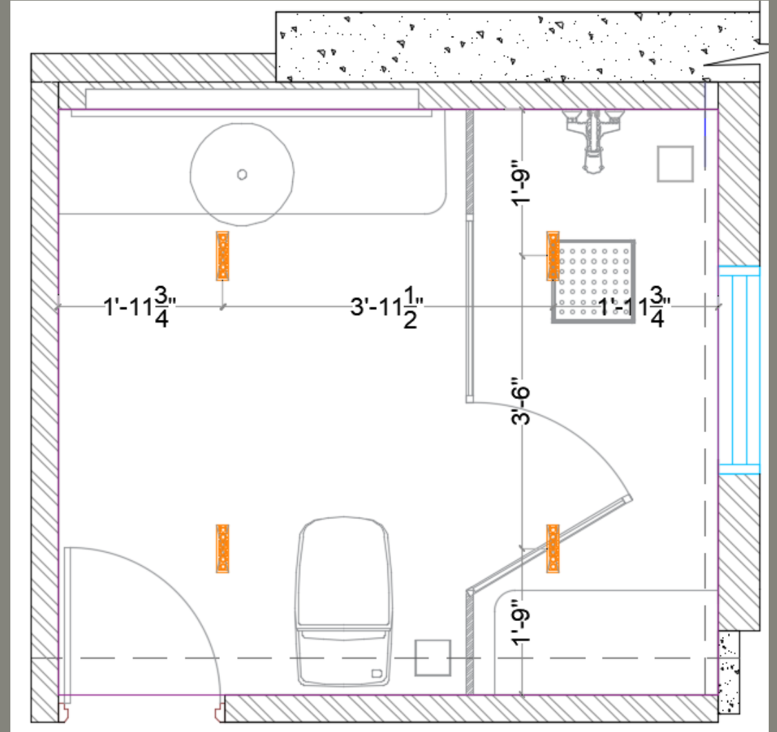
ELECTRICAL PLAN
