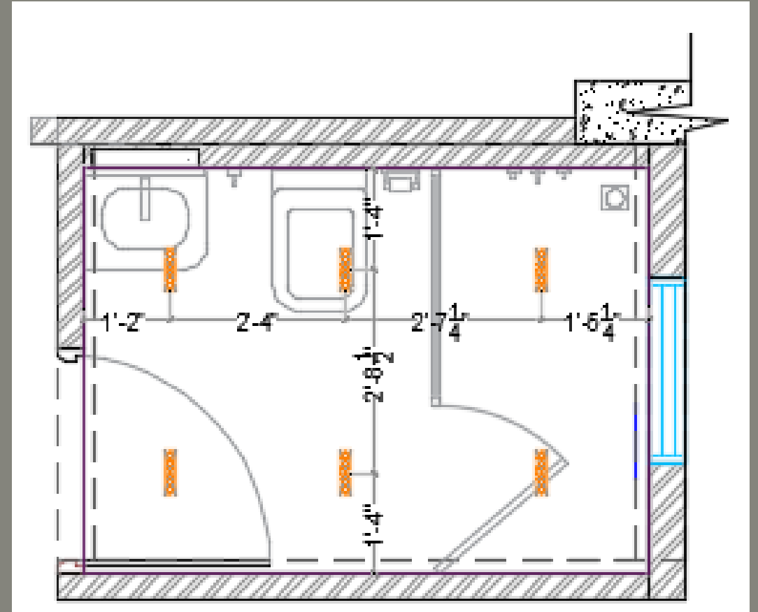
ELECTRICAL PLAN
