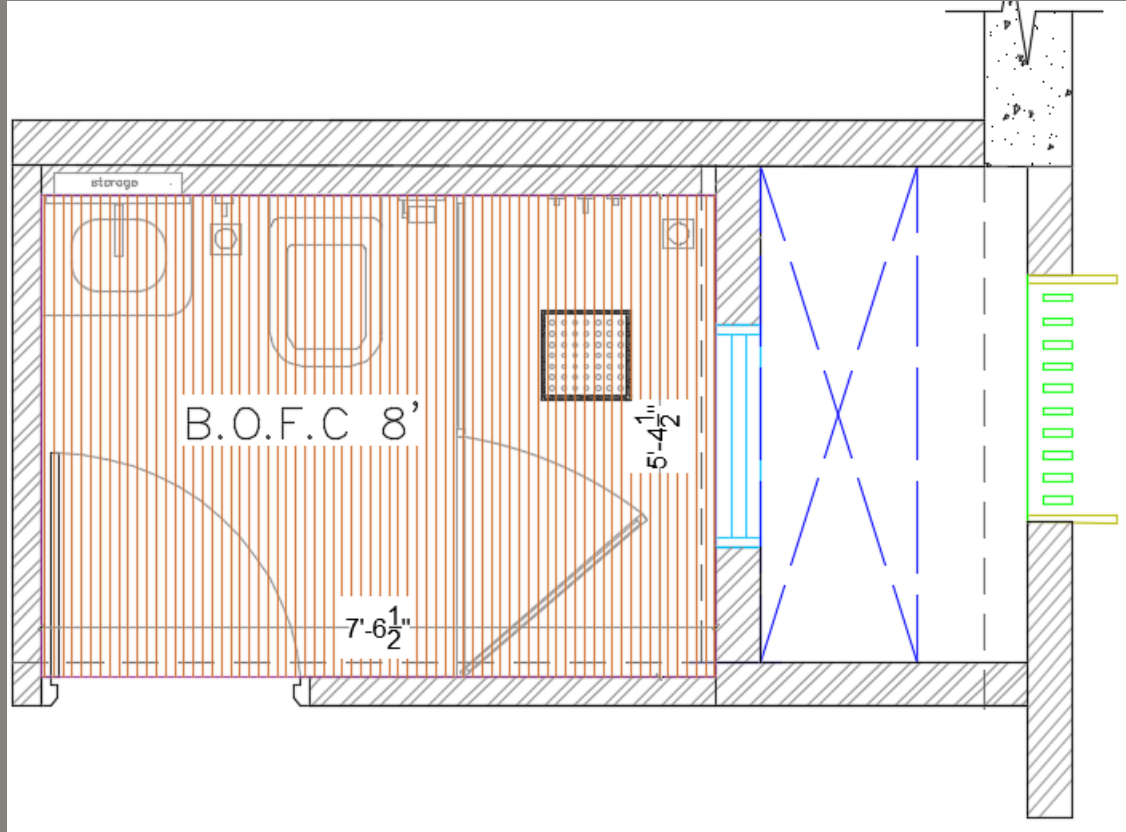
CEILING PLAN
