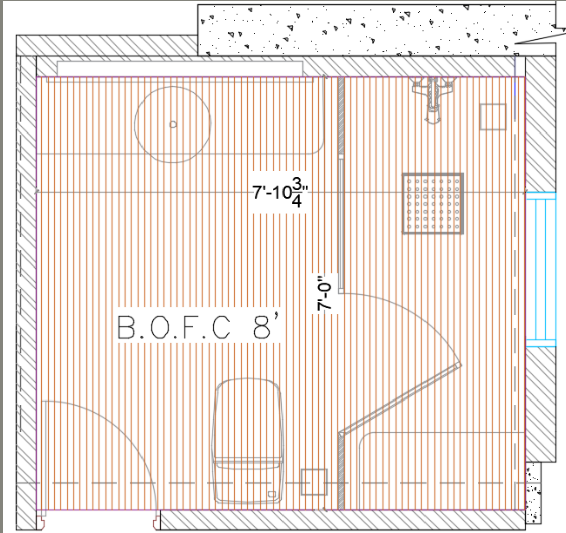
CEILING PLAN
