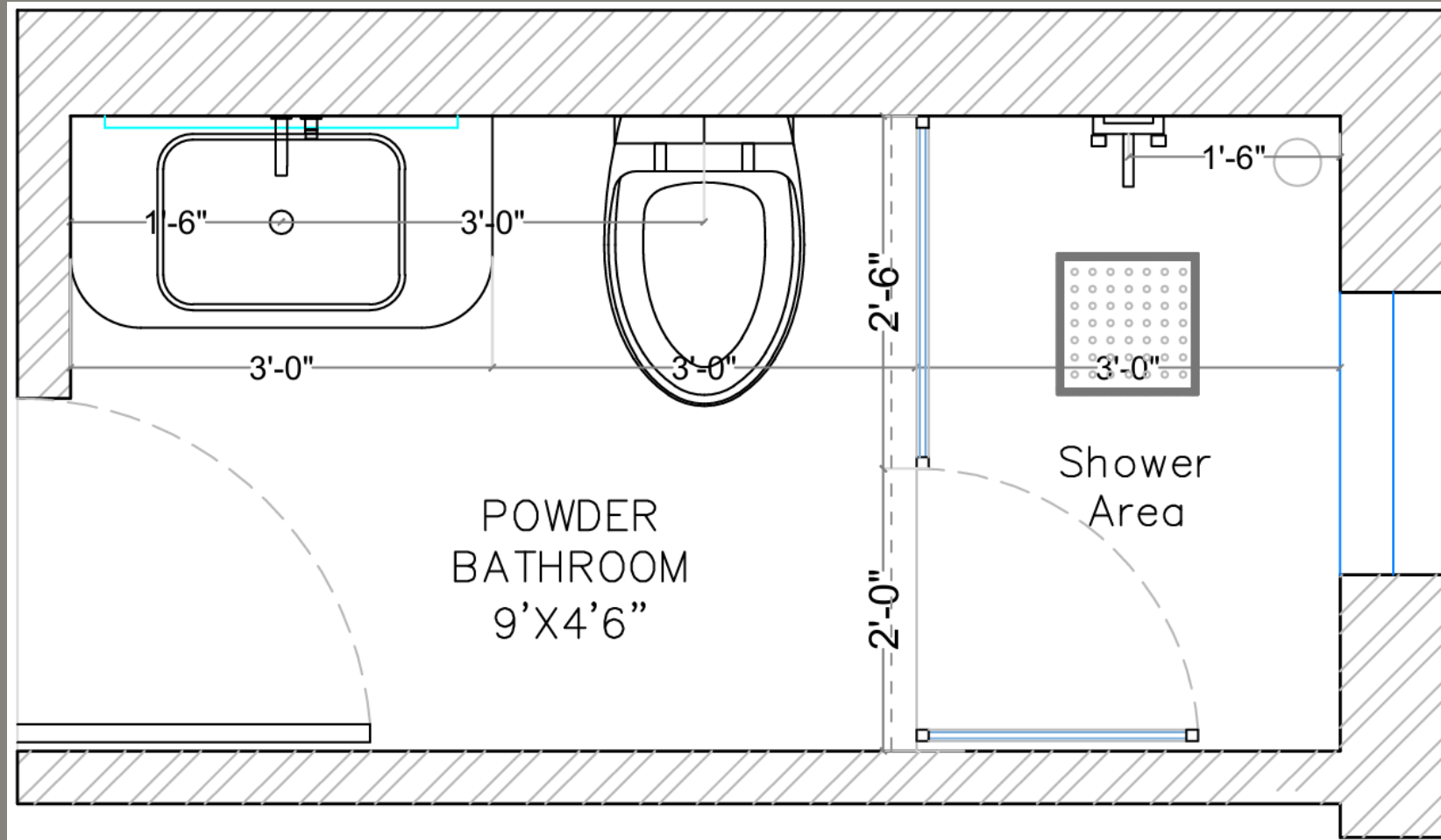
BATHROOM LAYOUT
