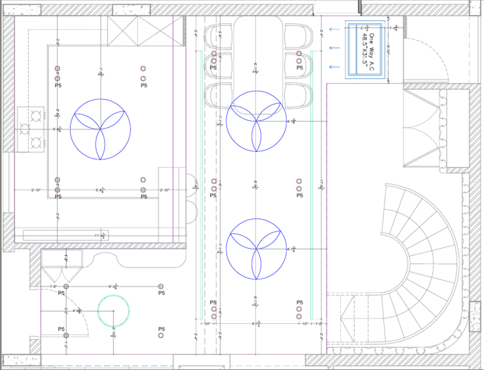
ELECTRICAL LAYOUT
