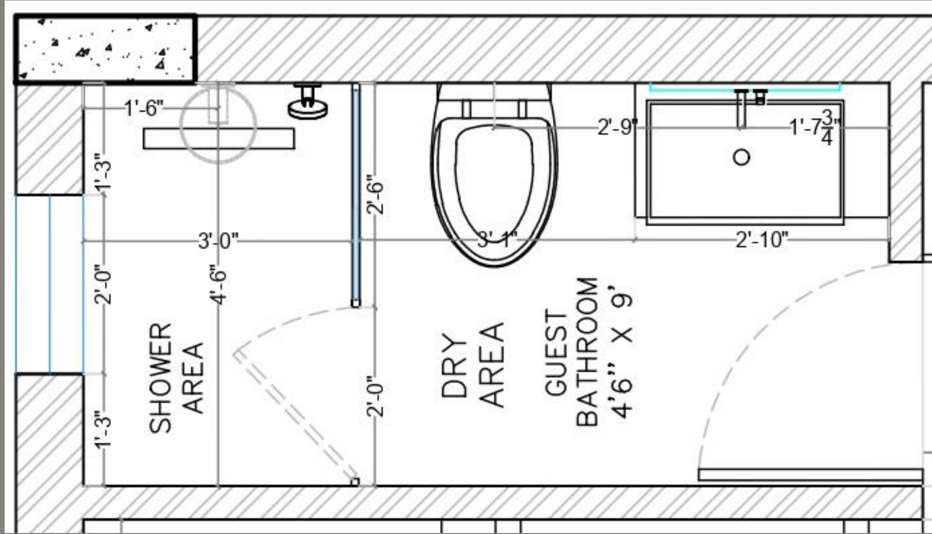
BATHROOM LAYOUT
