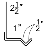
WINDOW/DOOR HEADER w/ GUTTER
