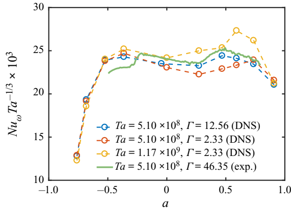
FIGURE 9. Compensated Nusselt number as a function of a obtained from the DNS of the current study. The green solid line is the experimental data performed at Ta = 5.10 \times 10^8 .
