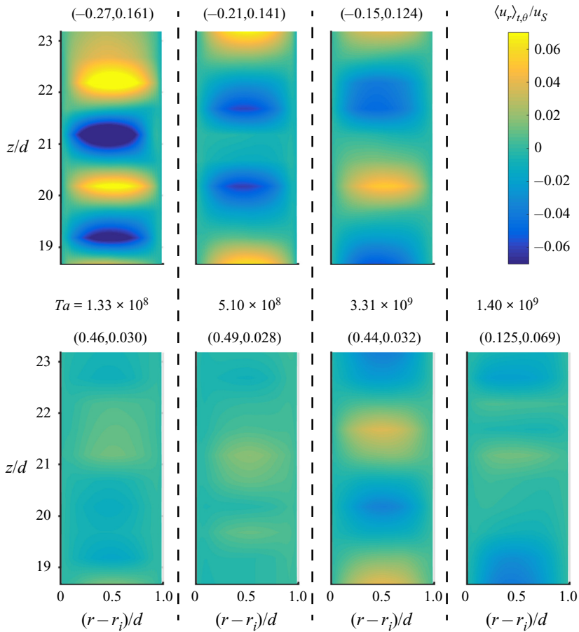
FIGURE 5. Azimuthally and time-averaged normalized radial velocity obtained from PIV experiments as described in figure 3. The legend on top of each figure represents the value of (a, R_\Omega) . The upper row represents measurements of the peak in the corotating regime while the bottom row shows measurements of the peak for counter-rotation. Along a single column, the Ta is fixed for both co- and counter-rotating states. The dashed lines are added to emphasize the difference between the Ta values.
