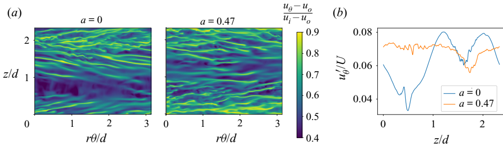
FIGURE 8. (a) Instantaneous normalized azimuthal velocity at r^+ = 15 for Ta = 5 \times 10^8 for a = 0 ( R_\Omega = 0.09 ) and a = 0.47 ( R_\Omega = 0.03 ). The DNS corresponds to the case of \Gamma = 2.33 . (b) Azimuthal average of the root-mean-squared azimuthal velocity u'_\theta as a function of axial position at r^+ = 15 for the two values of rotation a . A clear break in axial homogeneity can be appreciated for a = 0 .
