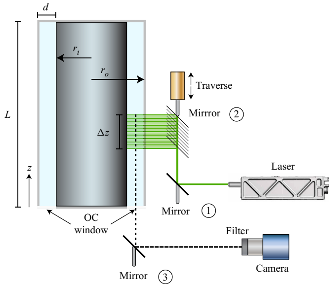
FIGURE 1. Sketch of the experimental set-up. All elements (except for the laser) are mounted on to the frame of the T 3 C. This results in no relative motion between the camera and the laser sheet due to mechanical vibrations. The velocity fields obtained with PIV are measured on the r - \theta plane.
