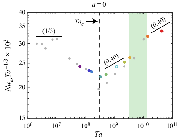
FIGURE 2. Compensated Nusselt number as a function of the driving strength Ta for the case of pure inner cylinder rotation a = 0 at \eta = 0.91 . The grey data points ( Ta < 10^8 ) correspond to DNS from Ostilla-Mónico et al. (2014b). The grey data points for Ta > 10^8 are also DNS simulations but from a different study (Ostilla-Mónico et al. 2014a). In addition, each coloured marker at fixed Ta corresponds to the driving variation as shown in the legend of figure 3(c). The open circle in light blue corresponds to the DNS data of the current study for \Gamma = 2.33 . The transition to the ultimate regime is observed at Ta = Ta_c \approx 3 \times 10^8 (vertical dashed line). The green shaded area corresponds to the region where a local change of slope can be seen due to the disappearance of quiescent wind shearing regions. The black solid lines serve as a reference to indicate the corresponding scaling.
