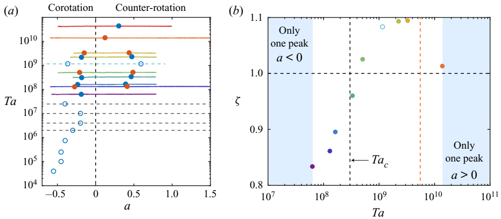
FIGURE 4. (a) Location in the phase space of the local maxima of angular momentum transport. The blue open circles for Ta \leq 2.5 \times 10^7 are the DNS of Ostilla-Mónico et al. (2014b). The blue open circles located at Ta = 1.17 \times 10^9 are from DNS of the current study. The solid circles represent experimental data for the local maxima of angular momentum. The solid orange circles represent turbulent states where we perform PIV experiments as described in § 4.3 and shown in figure 3. (b) Ratios of the magnitude of the angular momentum transport peaks as defined in (4.1). The coloured points represent the experimental data. The open circle represents the DNS simulation shown in (a) for Ta \approx 10^9 . The blue shaded areas represent turbulence levels wherein only one peak in angular momentum can be observed. The transition to the ultimate regime is observed at Ta = Ta_c \approx 3 \times 10^8 . The vertical red dashed line represents the prediction of Brauckmann & Eckhardt (2017) for the disappearance of the (broad) peak found in corotation, namely at Ta > 4.95 \times 10^9 .
