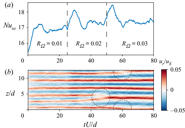
FIGURE 11. DNS results of varying R_\Omega for Ta = 5.10 \times 10^8 and \Gamma = 12.56 . (a) Temporal evolution of the dissipation Nu_\omega . (b) Time–space diagram of the instantaneous u_r at mid-gap. By looking at the regions of negative and positive radial velocities, which represent the outflow or inflow of rolls, two regions of merging rolls can clearly be seen. These mergers are highlighted with the dashed circles. The vertical dashed lines in (a) represent a stage during the simulation for a fixed value of R_\Omega .
