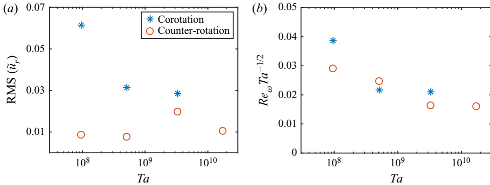
FIGURE 6. (a) RMS averaged along the axial direction of the azimuthally time-bulk-averaged radial velocity, normalized with the shear velocity u_S , as a function of the driving strength Ta . (b) Wind Reynolds number (based on the radial velocity) as a function of Ta . In both figures, the blue stars represent states that correspond to the peak in the corotating regime, while the red open circles represent measurements for the peak for counter-rotation.
