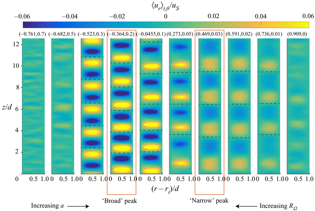
FIGURE 10. Azimuthally time-averaged radial velocity normalized with the characteristic velocity U obtained from DNS for Ta = 5.10 \times 10^8 and \Gamma = 12.56 . Each plot represents a different rotation state, quantified by either a or R_\Omega . The legend on top of each figure represents the value of (a, R_\Omega) . The flow state that corresponds to either the ‘broad’ or ‘narrow’ peak are highlighted in red. The arrows indicate the direction of the increment of either a or R_\Omega .
