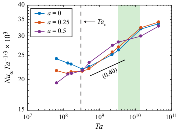
FIGURE 7. Compensated Nusselt number as a function of Ta for three rotation ratios. A reordering of the curves around Ta \approx 10^{10} can be seen. The green shaded area corresponds to the region where a significant change in the local scaling exponent can be seen due to the disappearance of quiescent wind shearing regions. The black solid line representing the scaling of Nu_\omega \propto Ta^{0.4} is given as reference.
