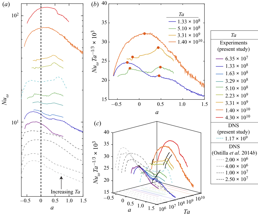
FIGURE 3. (a) Nusselt number Nu_\omega as a function of rotation ratio a for different values of the driving Ta . The vertical dashed line ( a = 0 ) in (a) separates the co- and counter-rotating regimes. (b) Compensated Nusselt number as a function of a for four selected Ta . Here, the solid red circles represent local maxima of angular momentum, where we perform PIV measurements as described in § 4.3. (c) A 3-D representation of the compensated Nusselt number as a function of Ta and a . The black solid lines represent the experiments performed for fixed a , i.e. Ta -sweeps. An animated version of this figure can be found in the Supplementary Material. In all figures, the solid lines represent experiments while the dashed lines represent numerics. The colours represent the variation in Ta as illustrated by the legend.
