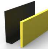
X50-KM10 (Wedge set for 5+5 mm Glass) X50-KM12 (Wedge set for 6+6 mm Glass) X50-KM16 (Wedge set for 8+8 mm Glass)
