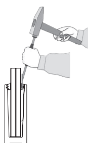
AK-5299 Wedge Fixing Tool
