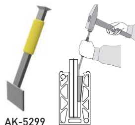
AK-5299 Wedge Fixing Tool
