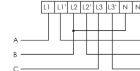
Fig 4 Three phase three lines direct connect
