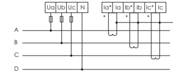
Fig 1 Three phase four lines connect via CT
