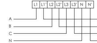
Fig 2 Three phase four lines direct connect
