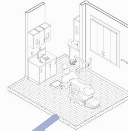
5 OPERATORY 120
