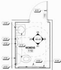
2 110 - WOMENS R.R. 3/8" = 1'-0"
