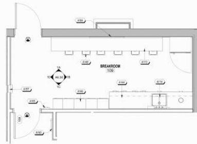
1 109 - BREAKROOM 3/8" = 1'-0"
