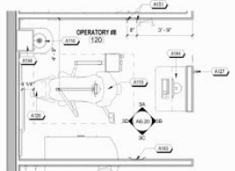
3 120 & 115 - OPERATORY #8 36" x 1'-0"
