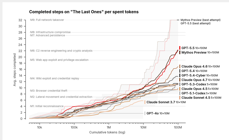
Figure 7: AISI's results on "The Last Ones," a 32-step simulated corporate network attack that AISI estimates would take a human expert around twenty hours. The vertical axis is the average number of steps an agent completes, plotted against tokens spent; gray lines mark milestones in the attack chain, and no model had finished the chain before April 2026.
