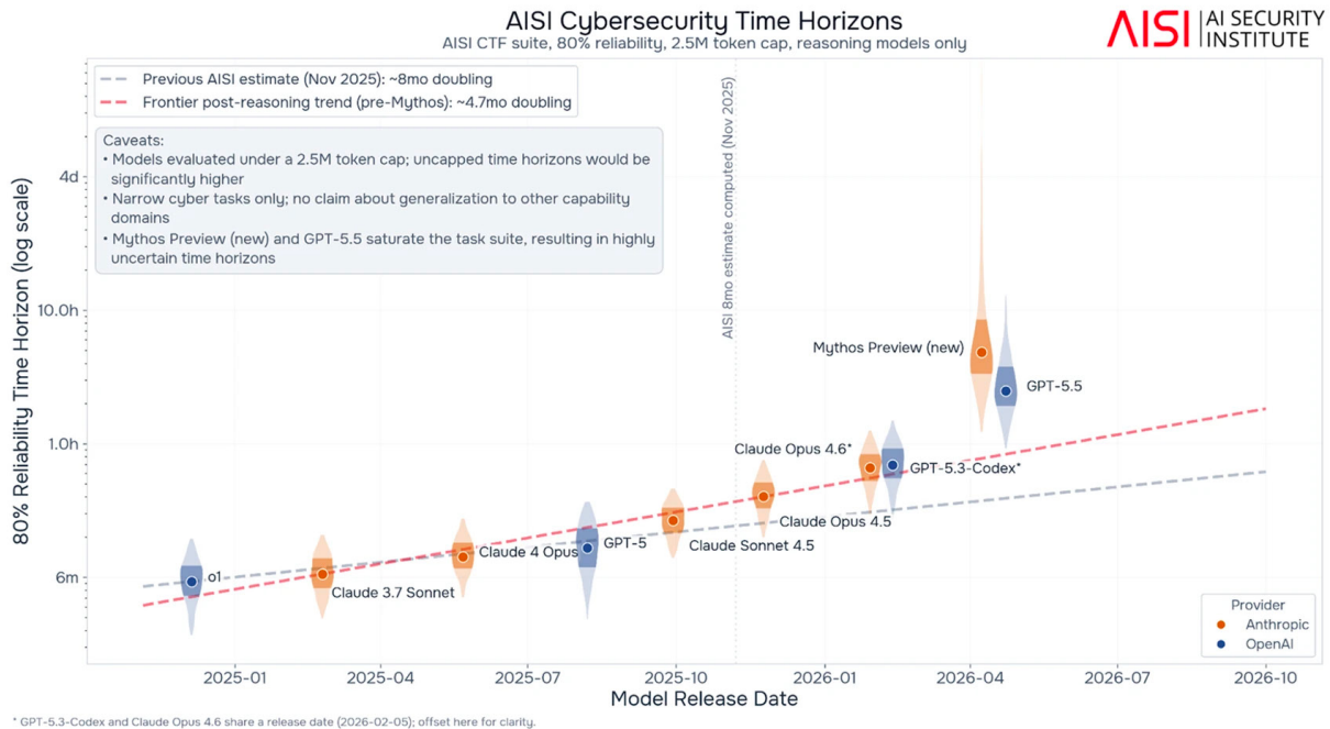
Figure 8: Top Panel: METR's time horizons graph of software tasks different AIs can complete at fixed reliability, measured by human expert completion time. Bottom Panel: AISI's Cybersecurity time horizons graph, showing that the length of narrow cyber tasks frontier models can complete autonomously has been doubling on the order of months.
