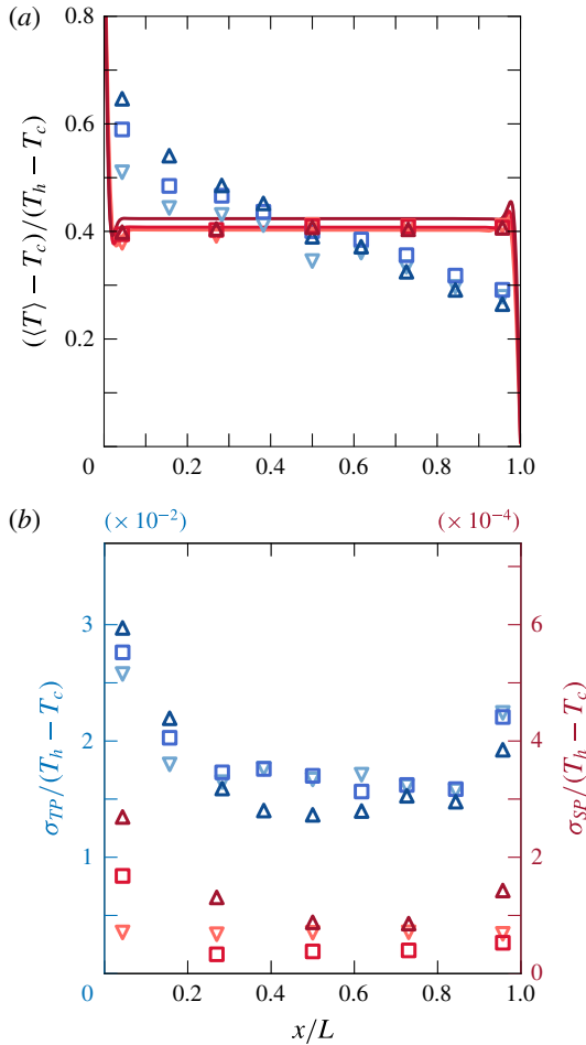
FIGURE 9. (Colour online) (a) Normalised mean temperature profile at the mid-height. The overshoots close to the walls in the numerical data appear because the thin layer of warmed up (cooled down) fluids moving upward (downward) are still colder (hotter) than the bulk where there is a stable stratification. (b) Normalised standard deviation of the temperature fluctuations. Red lines (numerical results in a ) and symbols (experimental data) represent the single-phase case and blue symbols the two-phase case with \alpha = 0.9\% , for various Rayleigh numbers: Ra_H = 5.2 \times 10^9 (downward triangles), Ra_H = 1.6 \times 10^{10} (squares) and Ra_H = 2.2 \times 10^{10} (upward triangles).
