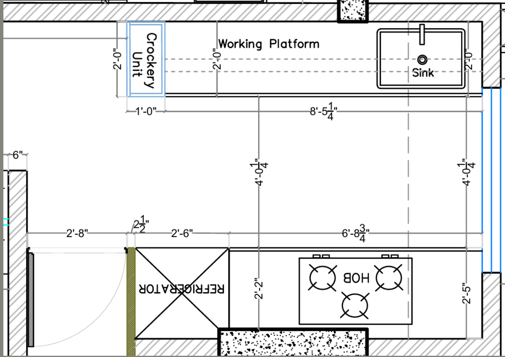
PLAN
