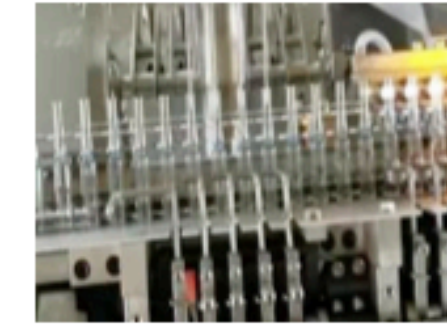
Processing Machine: Ampoule Filling Machine Control: PLC Origin: India
