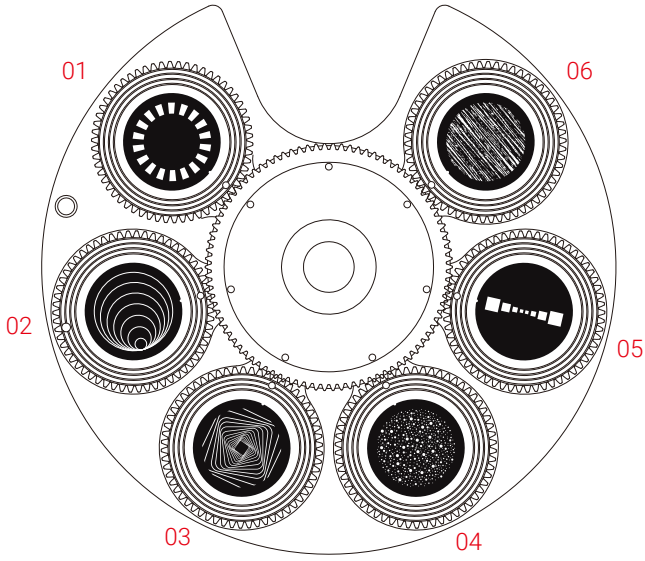
Rotating GoboWheel 1
