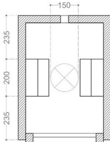
Section
