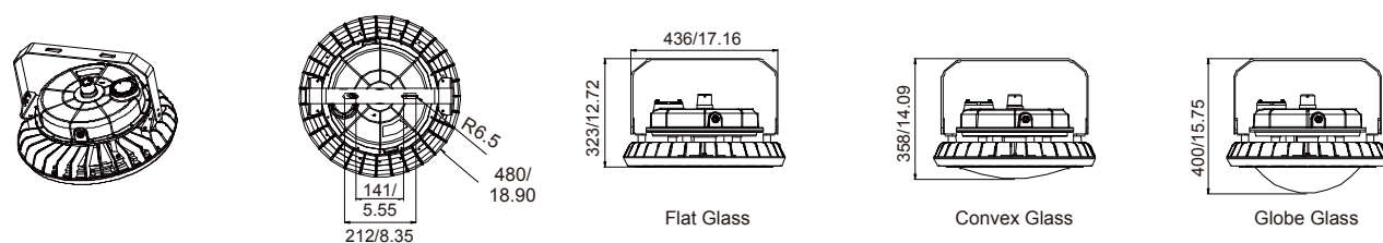
B4 with driver cover G and bracket
