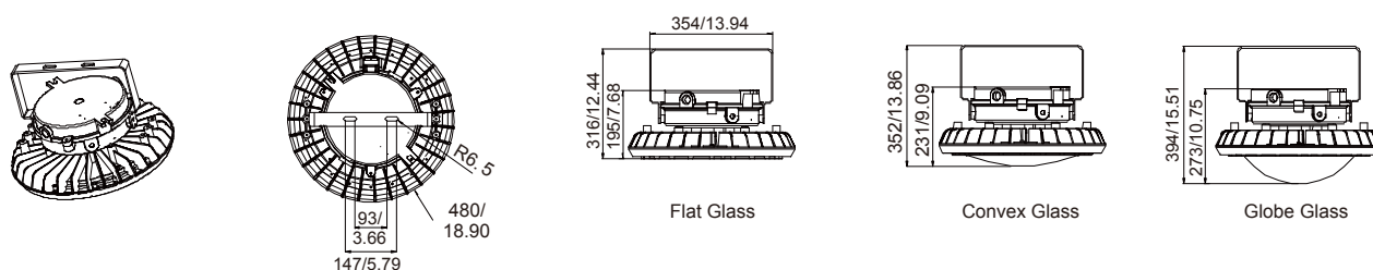
B4 with driver cover E and bracket
