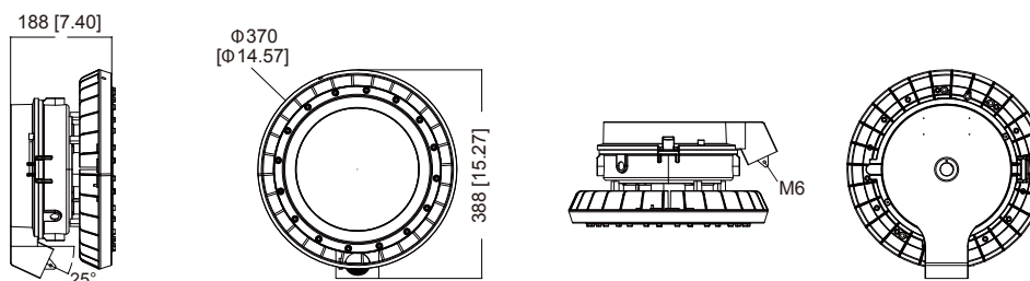
B3 with driver cover D, wire guard and flat diffuser
