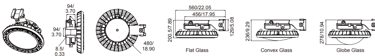
B4 with driver cover D
