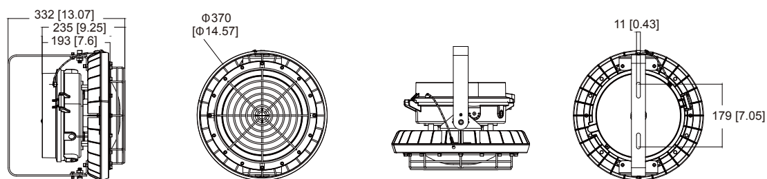
B3 with driver cover B, wire guard, convex diffuser (glass or PC), and bracket
