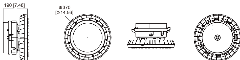
B3 with driver cover B and flat diffuser
