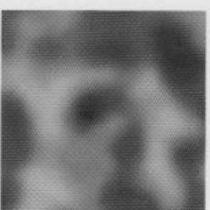
10^{-17} meters 0.01 fermis
