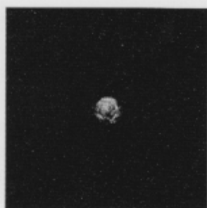
10^8 meters 100,000 kilometers
