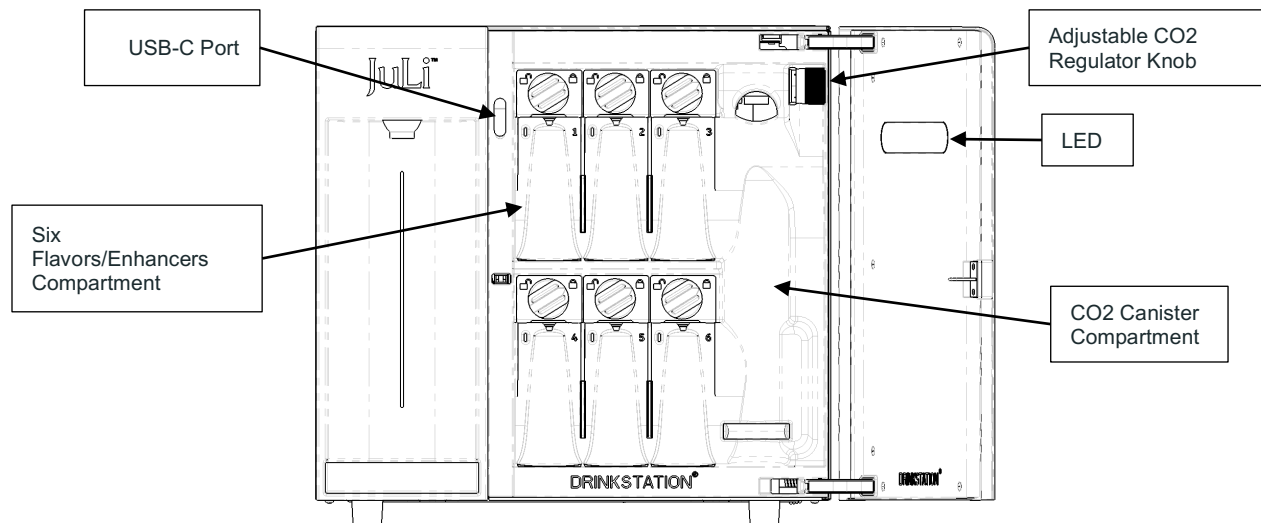
FIG. 2 JuLi 5.0 — Interior Layout (flavor compartments, CO2, ActiFilter and Mineral Alkaline Chamber pH+)
