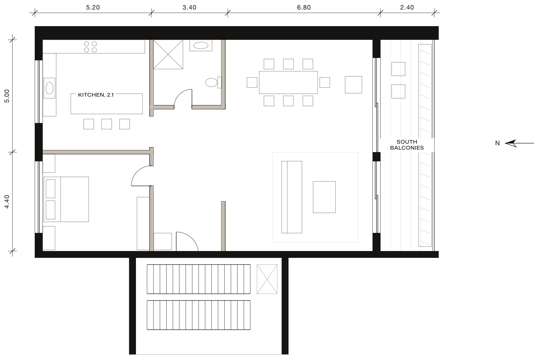
FLAT 2.1 — TYPICAL FLOOR, TYPE .1 (FLATS 1.1–3.1)
