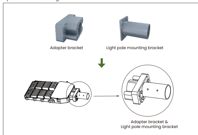
Option 3: Arm Mounting (A)
