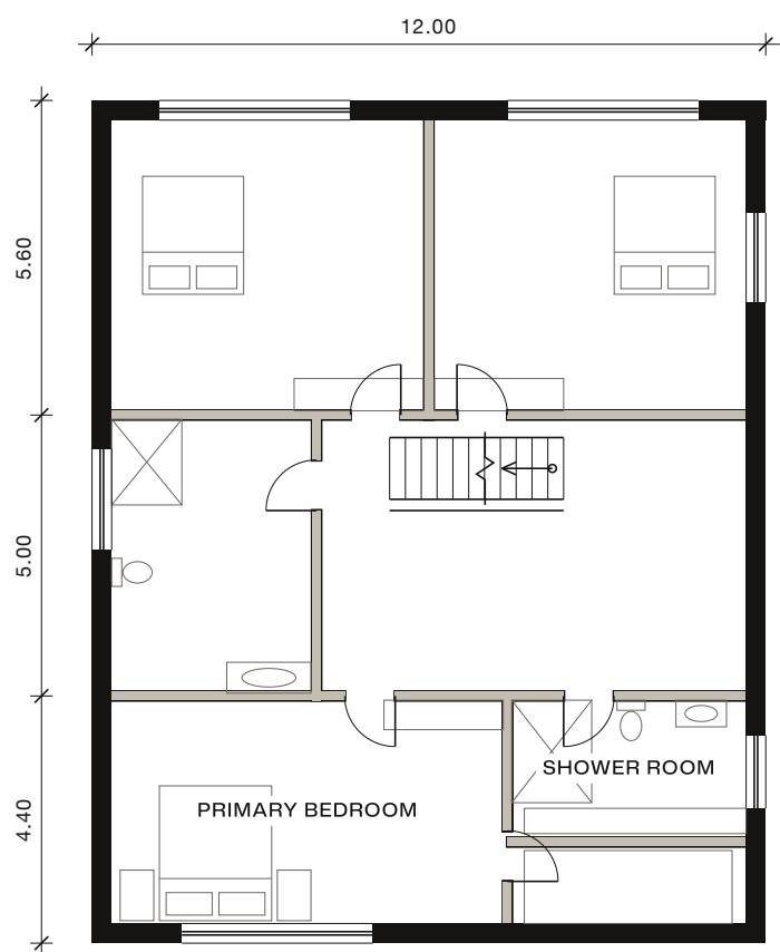
UPPER FLOOR
