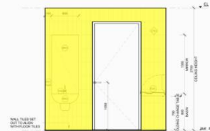
4 DISABLED - ELEVATION C 1:20
