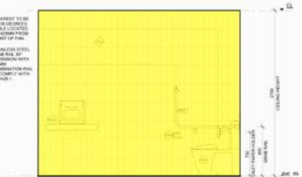
5 DISABLED - ELEVATION D 1:20
