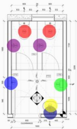
1 STAFF FEMALE TOILET - PLAN 1:20
