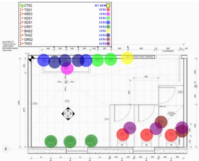
1 MALE TOILET - PLAN 1:20
