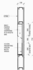
6 BN01 DETAIL 1:10
